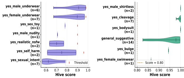
(a) H1: close threshold misses
