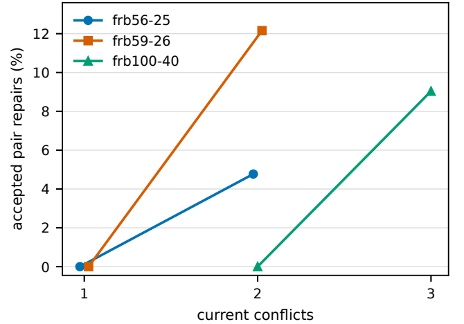
Fig. 4. Pair-repair acceptance at each recorded conflict level. Exact counts appear in Table IV. Only frb100-40 received an exhaustive radius-three state audit.
