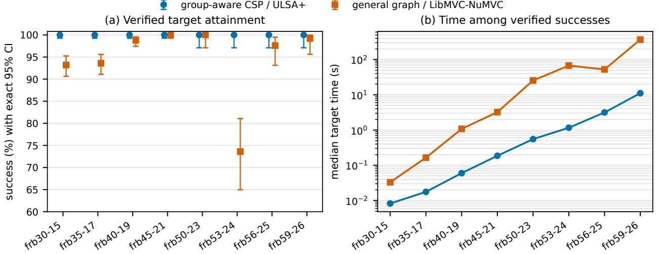
Fig. 2. A1 pipeline comparison by FRB family. (a) Verified success proportions with exact 95% binomial intervals. (b) Median target time among verified successes on a logarithmic scale; the medians exclude censored NuMVC runs. Solver, representation, and implementation vary together; the panels therefore summarize complete-pipeline performance.
