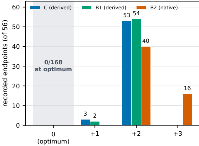
Fig. 3. Endpoint objective gaps in the three preregistered validation arms ( n = 56 per arm). No arm produced a verified certificate (0/56 in each; exact two-sided 95% CI 0–6.38%), so the planned hazard ratios remain unidentified. C and B1 gaps are reconstructed post hoc from recorded assignments and independently verified; B2 gaps are NuMVC’s reported cover values minus 3,900.
