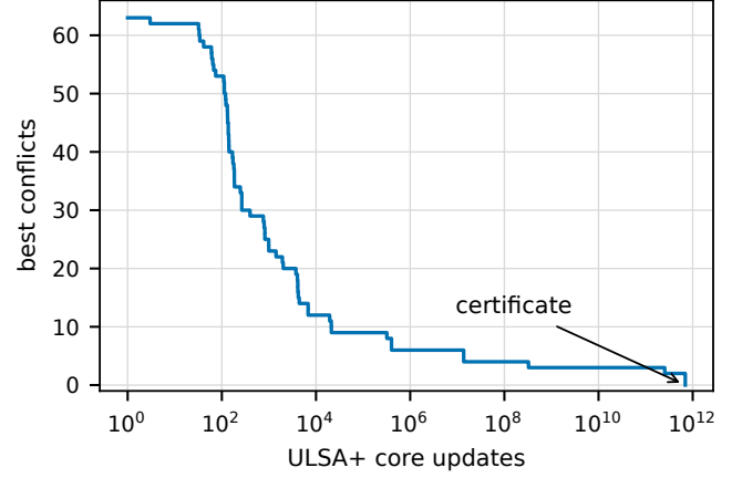
Fig. 1. Best violation count in the successful discovery process. The horizontal axis is symmetric-log scaled to retain the early transient and the long conflict-two tail.
