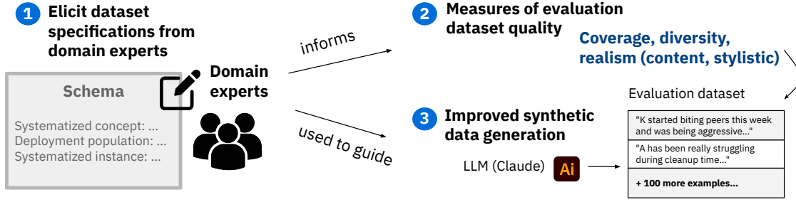
Figure 1: Study Contributions: An end-to-end approach for generating valid evaluation data at scale This paper makes three key methodological contributions: First, we introduce a schema: a lightweight, structured template that can be used to elicit key information about the intended scope and goals of the AI evaluation task. Second, we build upon past work to motivate and define four criteria for measuring the quality of evaluation data: coverage, diversity, content realism, and stylistic realism. Finally, we build upon these steps to show how the schema and quality metrics can be used to improve the quality of synthetic data generation for AI evaluation.
