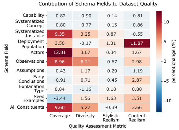
Figure 2: Percent contribution of each schema field to the four dataset quality criteria. Coverage and Content realism are most affected by specific fields in the schema, followed by Diversity. Stylistic realism does not rely on any particular field. This figure shows that if the systematized instance or all constituents are not specified, coverage could drop on average 9% in the social work context.
