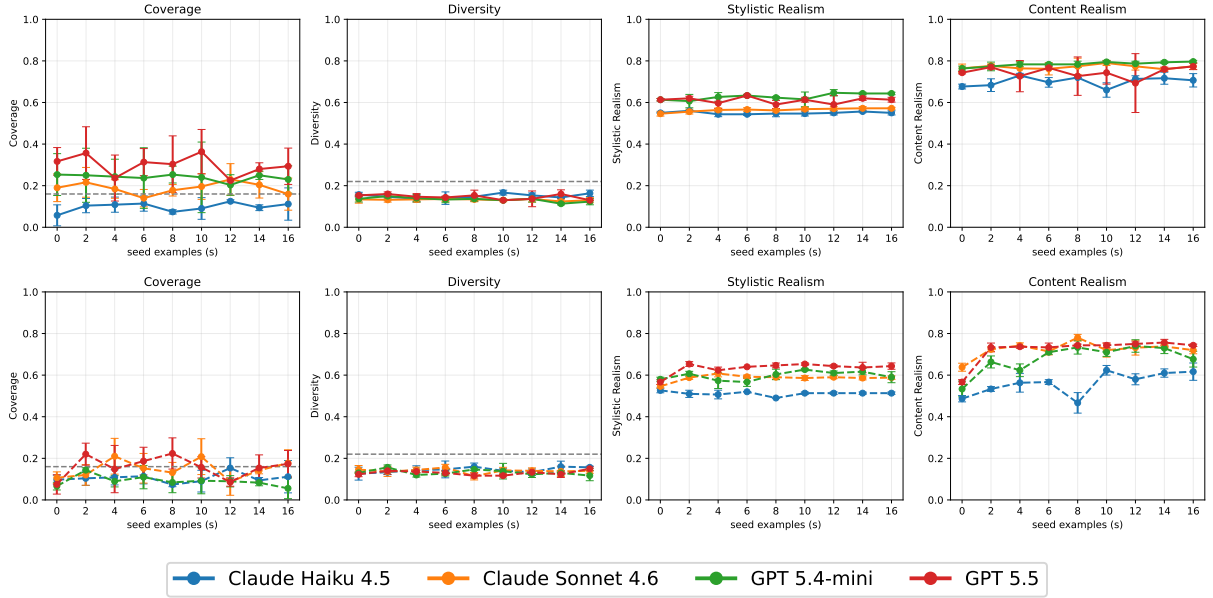
Figure 4: Different generation models across varying number of seeds. All points represent a mean over five runs, error bars represent standard deviation with the schema-generated dataset results on top and the baseline on the bottom. The horizontal gray dashed line indicates the 16 seed example’s coverage and diversity.
