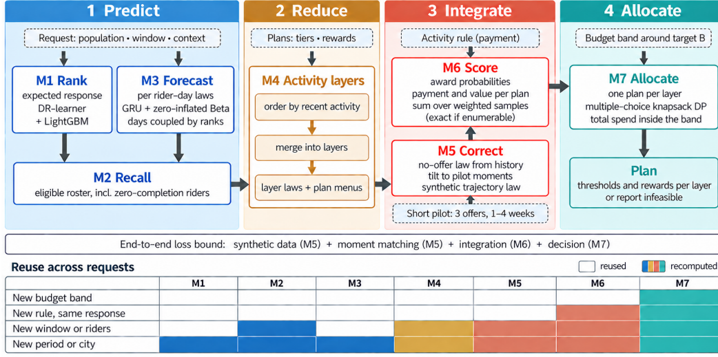
Figure 1: Request-driven framework: four stages and seven modules. Dashed chips are inputs (request fields, candidate plans, activity rule, budget band, short pilot); arrows show data flow between modules. Predict (M1–M3) gives every eligible rider a conditional completion law; Reduce (M4) merges riders into activity layers with plan menus; Integrate (M5–M6) tilts the no-offer law to short-pilot moments and scores every plan by a weighted sum over stored samples of the corrected law, an exact sum when the trajectory types can be enumerated; Allocate (M7) chooses one plan per layer inside the two-sided budget band and returns the rewards that attain it. The bar names the four terms of the end-to-end bound (Proposition 1); the table marks what a new request recomputes.
