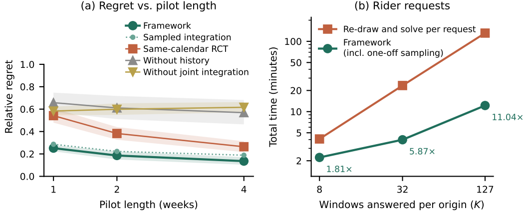
Figure 2: (a) Relative regret against pilot length, 18 response laws, 10% scoring; bands: 95% intervals over laws. (b) Total time to answer K windows per origin on rider records, one-off sampling pass charged; labels: median paired speed-ups.
