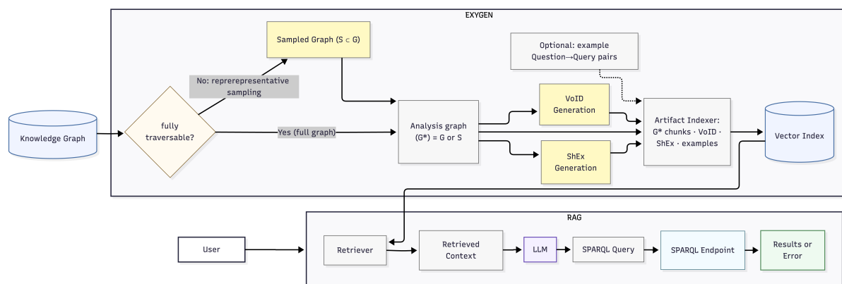
Figure 1: The EXYGEN-RAG pipeline. EXYGEN (top) ingests a KG and produces VoID and ShEx artifacts – via full traversal or representative sampling for large graphs – indexed for semantic retrieval. The RAG component (bottom) retrieves these artifacts at query time to guide an LLM in generating and executing SPARQL queries against the KG.
