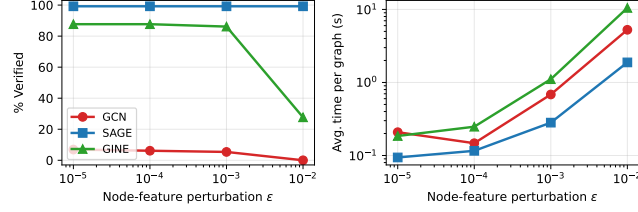
Fig.3: GNNV verification on IEEE-24 power flow across three architectures (GCN, SAGE, GINE-Conv) vs. node-feature perturbation \epsilon (log axis). (Left) percentage of voltage-magnitude nodes verified. (Right) average verification time per graph instance (log scale).
