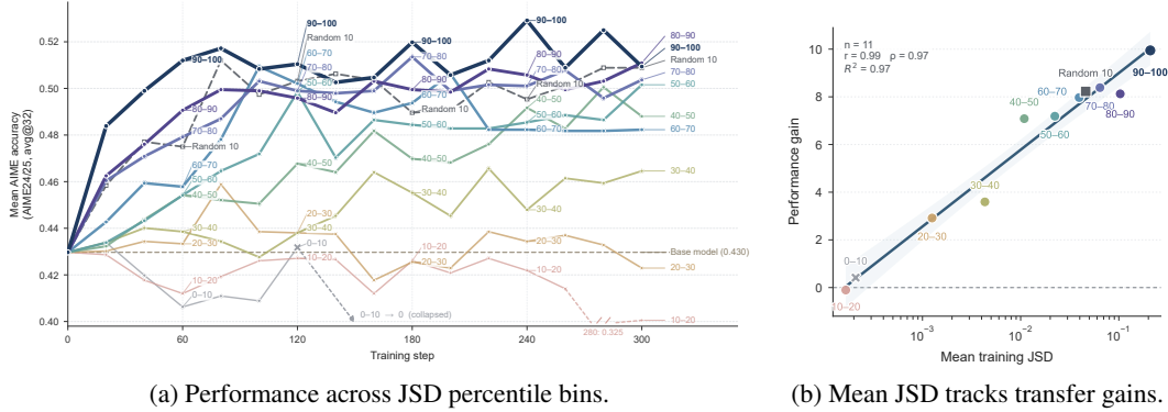
Figure 3: Which states are retained, not how many, determines transfer (Qwen3-1.7B, JustRL teacher pair). (a) Validation accuracy when training on each JSD percentile bin or on a random 10% of states. (b) Gain in peak validation accuracy over the initial student versus the mean training JSD of the retained states; the line is a log-linear fit.
