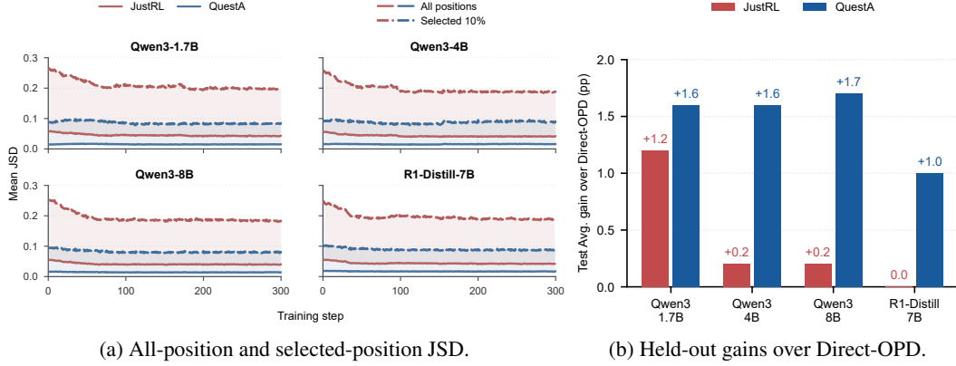
Figure 4: Teacher-pair comparison with top-10% retention across four students. (a) Mean teacher-reference JSD over all valid response states (solid) and retained states (dashed) during S^2D -OPD training. (b) Held-out Test Avg. gains of S^2D -OPD over dense Direct-OPD under each teacher pair, in percentage points.
