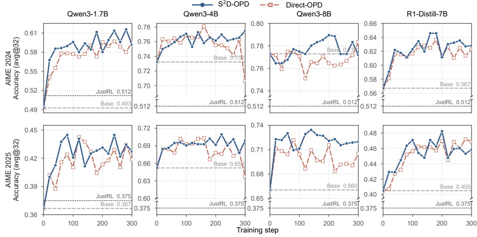
Figure 2: Validation accuracy (Avg@32) under the JustRL teacher pair across four students. Dashed lines mark the initial student; dotted lines mark the JustRL-1.5B teacher.
