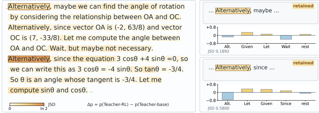
Figure 10: Retained shifts encode continuation preferences. At two retained states, the teacher shifts probability away from Alternatively ; the later state favors Let , Given , and Since .
