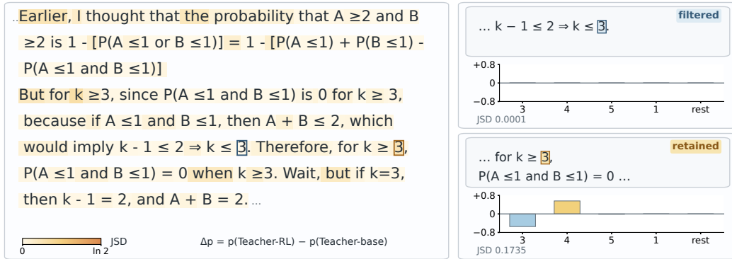
Figure 9: Same sampled token, different mask decisions. The mask filters a calculation on which the teacher and reference agree but retains supervision for a boundary correction.
