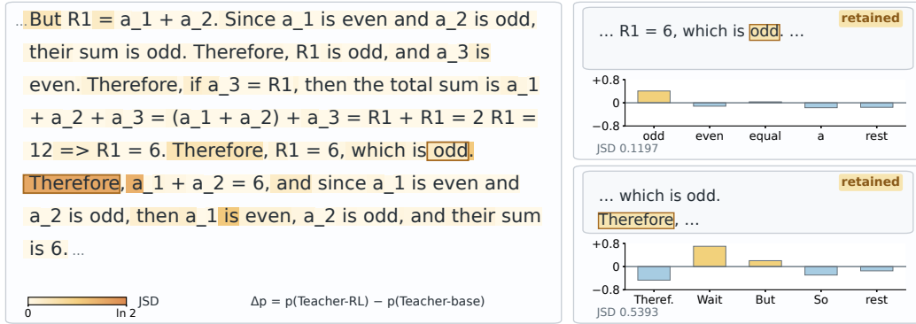
Figure 11: A later reconsideration cue does not undo an earlier adverse shift. The mask retains a shift toward an incorrect parity judgment, followed by a teacher preference for reconsideration.
