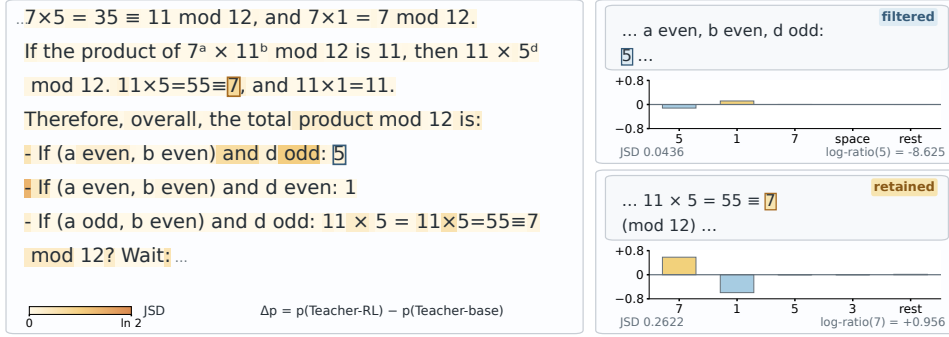
Figure 5: JSD and token log-ratio rank states differently. The state with the largest sampled-token log-ratio in the response is masked, while a larger redistribution of probability mass is retained.
