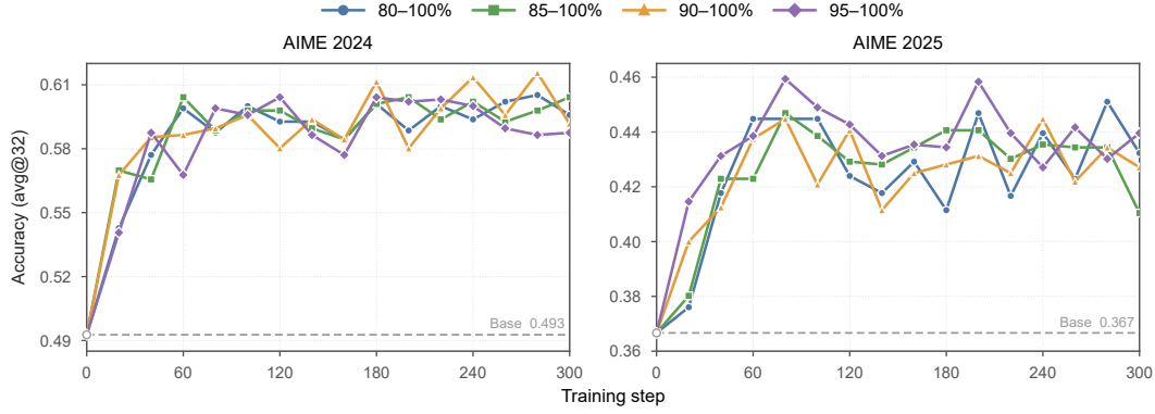
Figure 8: Sensitivity to the per-response retention ratio for Qwen3-1.7B under the JustRL teacher pair. The four settings retain the top 20%, 15%, 10%, and 5% of positions ranked by teacher-reference JSD. Dashed lines indicate base-model accuracy.
