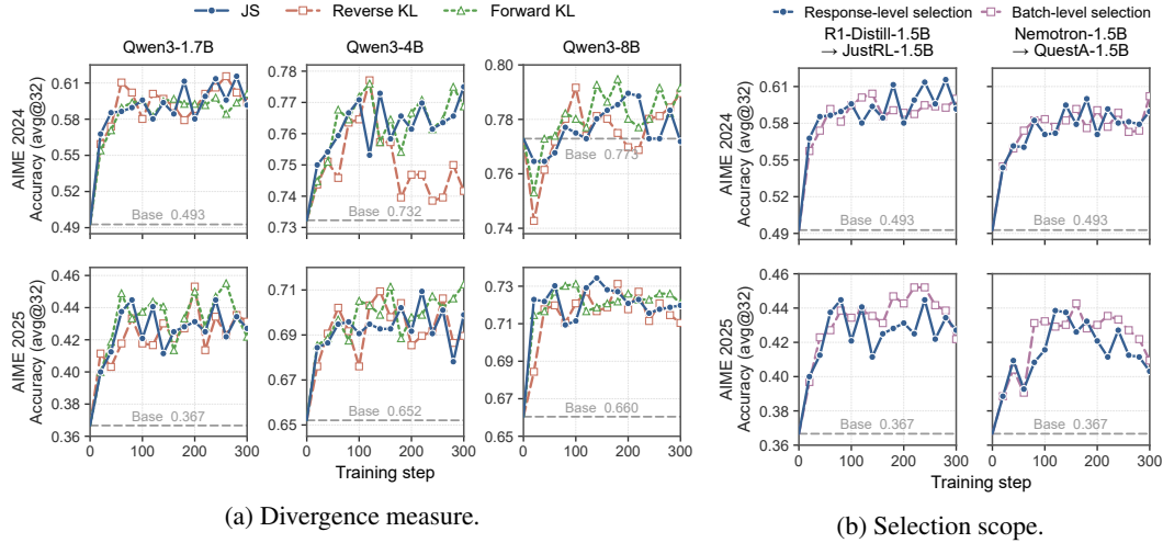
Figure 6: Robustness of selective masking across design choices. (a) Top-10% selection by JSD, reverse KL, and forward KL on Qwen3-1.7B, 4B, and 8B under the JustRL teacher pair. (b) Response-level versus batch-level selection on Qwen3-1.7B under both teacher pairs.
