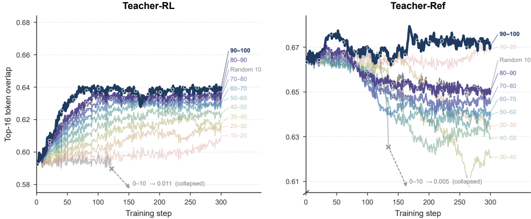
Figure 7: Top-16 token overlap over training for Qwen3-1.7B under the JustRL teacher pair, using JSD deciles or random 10% selection. Panels compare the student with the post-RL teacher (left) and pre-RL reference (right). Overlap is the fraction of shared tokens between top-16 sets.
