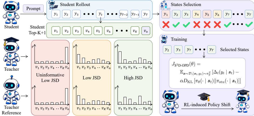
Figure 1: Overview of S^2D -OPD. At each student-sampled state, teacher–reference JSD is computed over the student’s top- K candidates, with the remaining probability mass grouped into a residual token v_0 . The highest-JSD states within each response are retained for the Direct-OPD objective.
