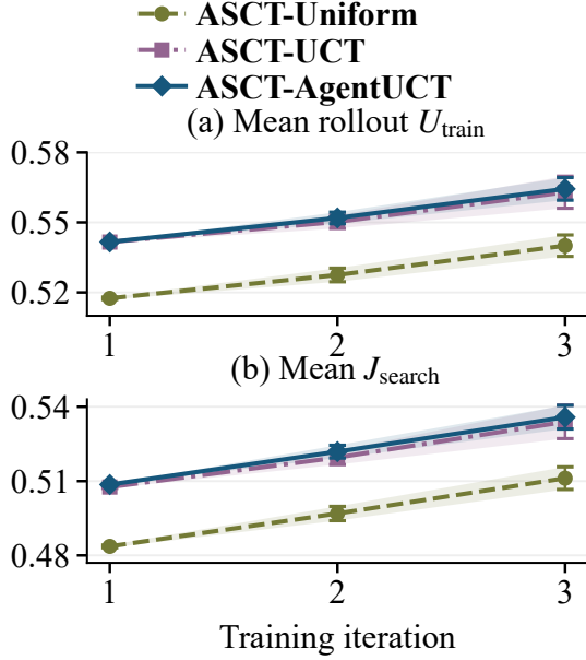
Figure 4: Per-iteration auxiliary evaluation within ASCT: mean rollout U_{\text{train}} and J_{\text{search}} (2,000 questions; B = 12 ). Utility uses the training scorer. Bands and bars: \pm sample SD across three seeds.
