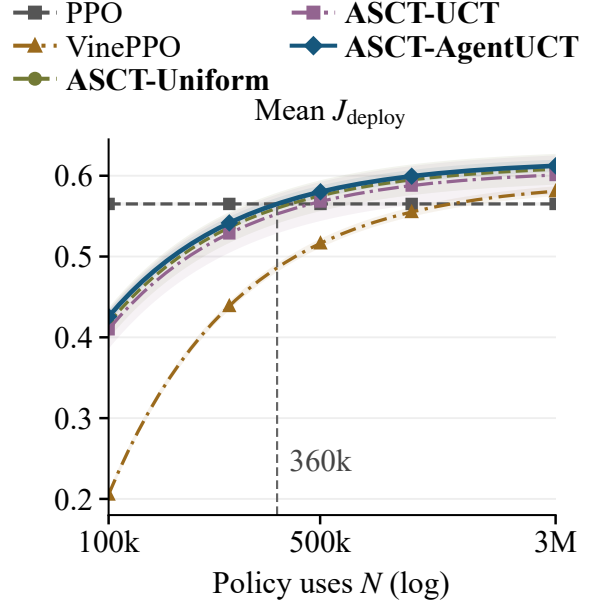
Figure 5: Amortized value across assumed policy uses N (Equation 6; \beta = 10^{-4} ). Bands: \pm sample SD across three seed projections. The guide marks AgentUCT's mean crossing with PPO. Both J metrics charge the recorded auxiliary ledger.
