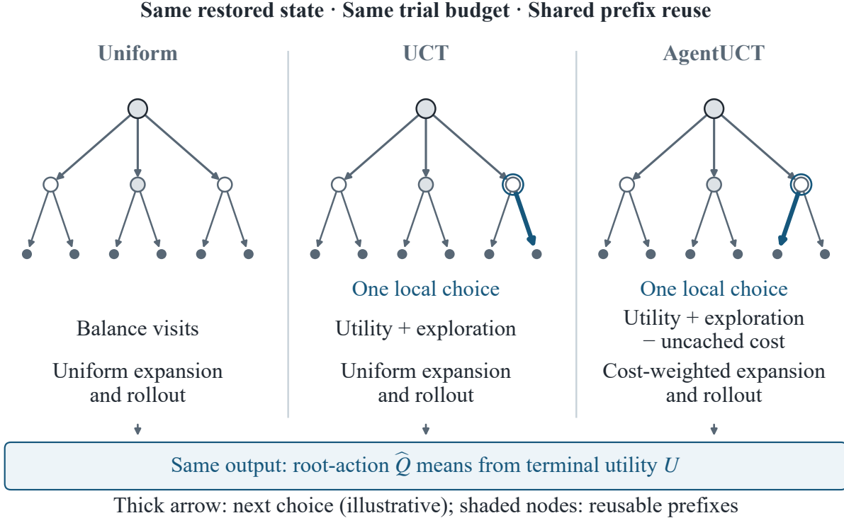
Figure 8: Decision rules within the three ASCT evaluators. UCT and AgentUCT share the depicted tree and prefix; the thick arrow differs only at one circled internal node, illustrating a possible local change in the next choice. Arrow thickness does not encode visit counts or the frequency or magnitude of cost effects. AgentUCT adds predicted uncached cost to selection and uses cost-weighted sampling. All three use WTB prefix reuse, back up terminal utility U , and return root-action means (Li et al., 2026).
