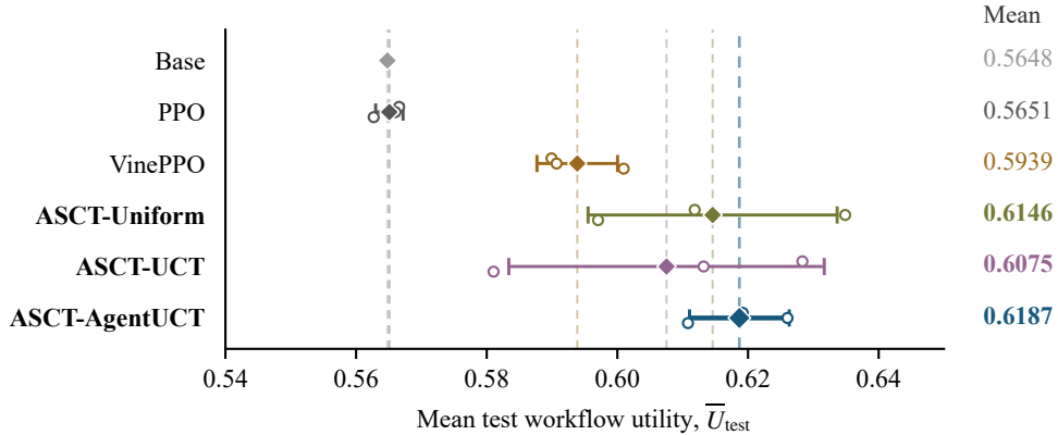
Figure 2: HotpotQA test utility. Diamonds and dashed guides mark means; bars show \pm 1 sample SD over three seeds; open circles show seeds. Base is fixed; ASCT labels are bold.
