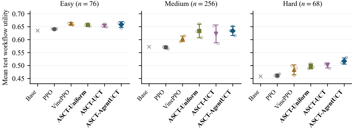
Figure 3: Test utility by difficulty: mean \pm sample SD over three seeds, with open seed markers. Base is fixed. Panels share the utility scale and method order.
