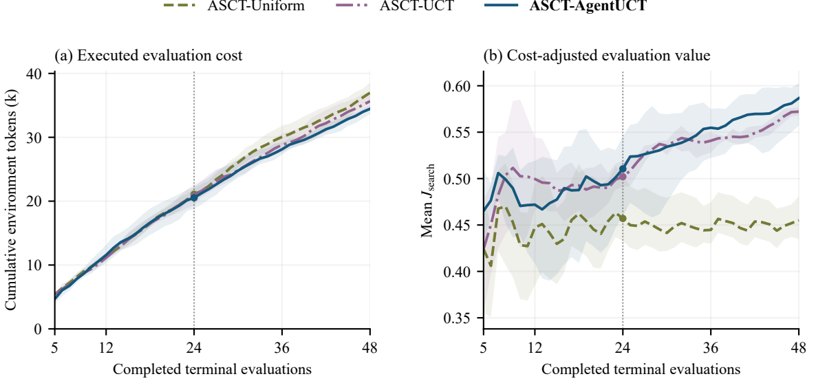
Figure 9: Executed auxiliary tokens and cost-adjusted evaluation value on the same states and budgets as Figure 6. \bar{J}_{\text{search}}(K) = \bar{U}(K) - 10^{-4}T_{\text{aux}}(K)/K . Auxiliary actor scoring is zero for these three evaluators, so total auxiliary cost equals environment cost. The deployment amortization curve uses Equation 6. Lines and bands follow Figure 6.
