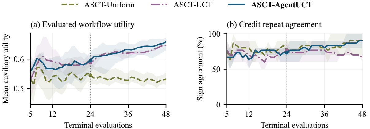
Figure 6: Fixed-state evaluation on two questions, three frozen actor seeds, and two repeats per state. Lines are seed means; bands span seed means. Credit agreement compares signs across repeats. All budgets from 5 to 48 are retained; the guide marks 24.
