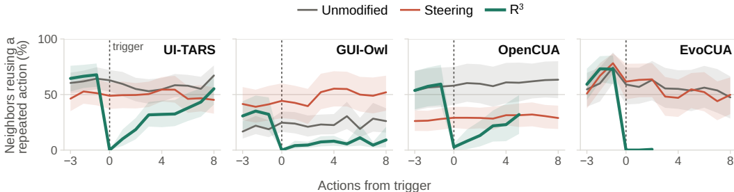
Figure 6: Activation neighborhoods after the first trigger. Share of the 25 nearest unmodified-agent activations associated with reuse of a previously unchanged-screen action. After reset, this share drops sharply at the trigger.
