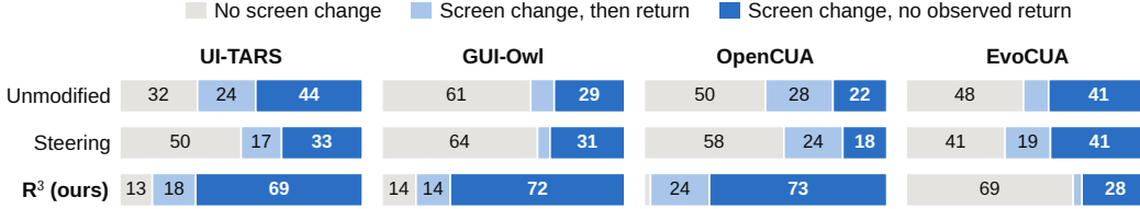
Figure 7: Screen changes and returns on OpenComputer. Percentages of all triggers, averaged over runs. A return repeats the original screen–action pair after a screen change and leaves the screen unchanged, within recorded follow-up.
