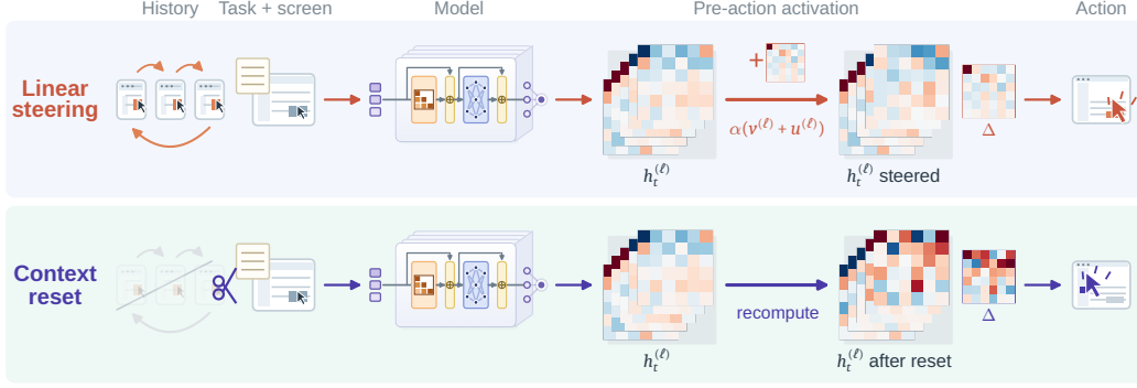
Figure 5: Editing pre-action activations. Steering edits the activation, while context reset removes the interaction history before recomputing it. Both rows show measured changes in activations for the two policies. Activations matrices are extracted from real data.
