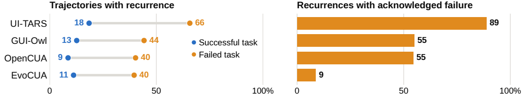
Figure 2: Recurrence concentrates in failed trajectories. Recurrence rate (%) by task outcome (left) and acknowledged share (%) of recurrences (right) per model. Data from both benchmarks are pooled.
