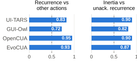
Figure 11: Validation AUC of the recurrence readout (left, OSWorld) and the inertia readout (right, both benchmarks). The dashed line marks chance.
