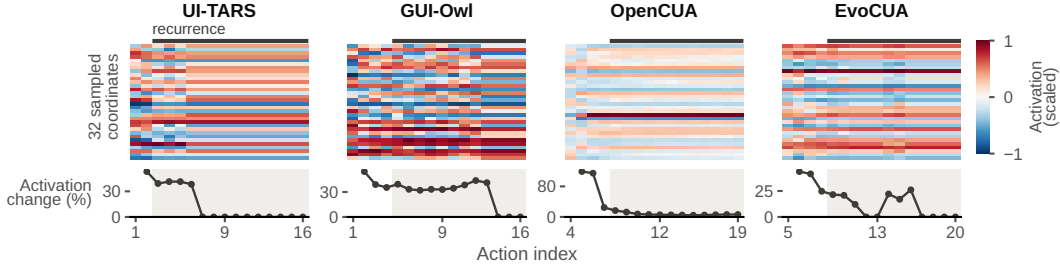
Figure 3: Activation persistence during recurrence. Top: normalized values of 32 sampled pre-action activation coordinates across consecutive actions; the black bar denotes the screen-action recurrence run. Bottom: change between consecutive activation vectors, measured relative to the model’s typical activation magnitude (the median vector norm in its reference sample).
