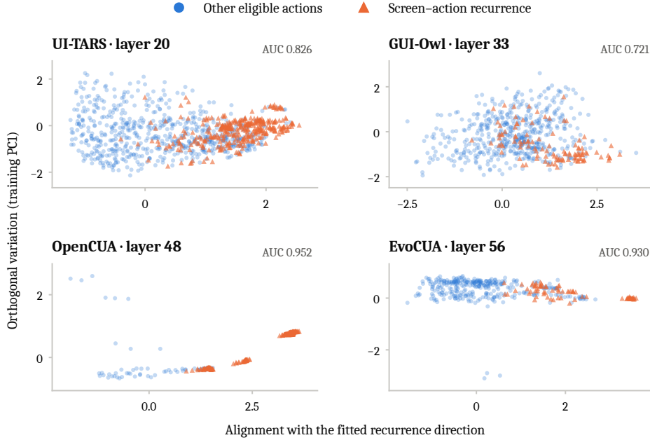
Figure 10: Validation actions projected onto the fitted direction v^{(\ell)} and orthogonal training PC1, in training standard deviations. AUC averages within-task comparisons on the data used to select layers. Density reflects action counts.
