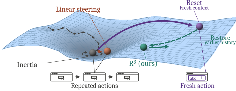
Figure 1: Activation editing of an absorbing region. In inertia, the agent remains near a repeated pre-action state. Linear steering can preserve this pattern, while context reset recomputes the state from a fresh context and can lead to a different action. R^3 restores the earlier history after finding a screen-changing action. Geometry and arrows are schematic.
