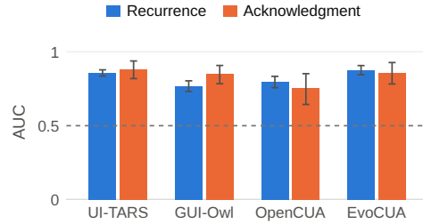
Figure 4: Activation readouts on held-out tasks. Mean AUC under nested task validation, with equal task weights. Error bars: 95% bootstrap intervals. Dashed line: chance.
