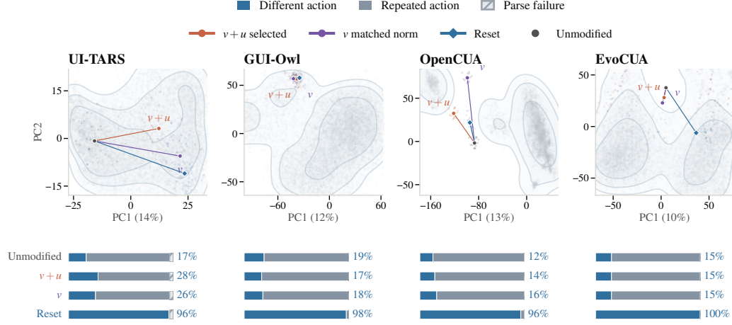
Figure 12: Activation movement does not always change the action. Task-weighted PCA of OSWorld reference states (gray) and OpenComputer interventions (colored). Lines join the unmodified mean to composite steering, matched-norm recurrence-only steering, and reset. Bars show all proposal outcomes; percentages count proposal escapes, not executed progress.
