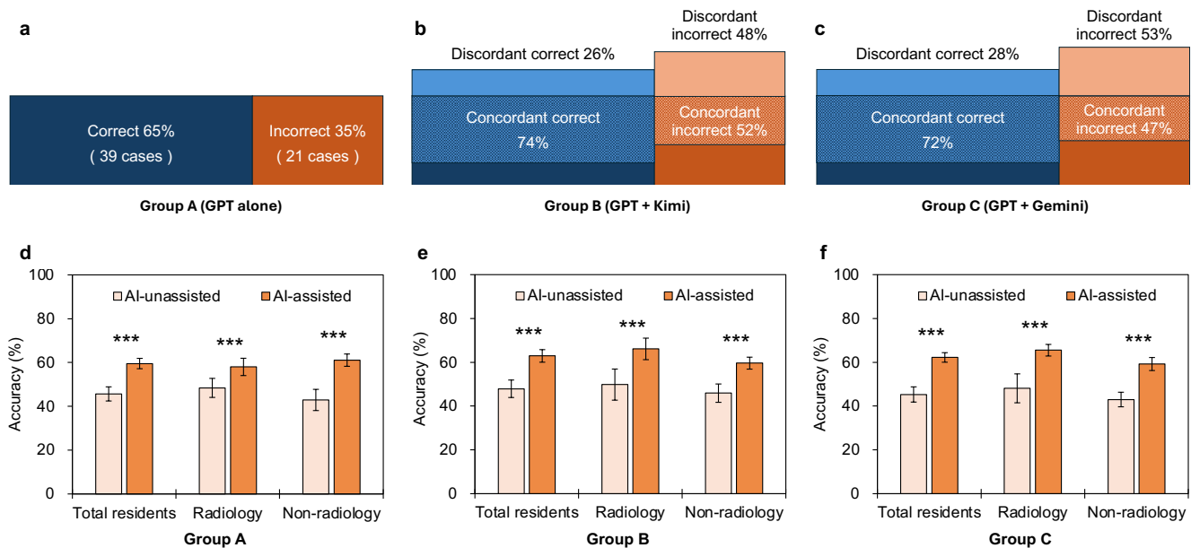
Figure 3. AI Model Concordance and Diagnostic Accuracy With and Without AI Assistance. a–c, AI diagnostic performance and case-level concordance in groups A–C. In the dual-suggestion groups, concordant and discordant categories indicate whether the second model agreed with GPT-5.4 among GPT-5.4-correct and GPT-5.4-incorrect cases. d–f, Mean AI-unassisted and AI-assisted diagnostic accuracy among all residents, radiology residents, and non-radiology residents in groups A–C. Error bars represent 95% CIs. *** P < .001 for paired comparisons between AI-unassisted and AI-assisted accuracy.
