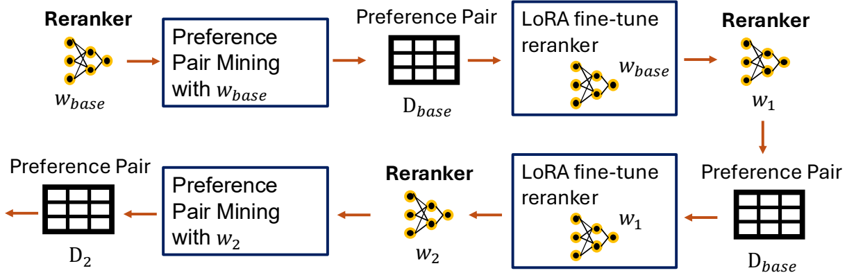
Fig. 3. Iterative preference alignment with periodic re-mining. Training begins with the base reranker weights w_{base} . Preference pairs are first mined under w_{base} , producing dataset \mathcal{D}_{base} . The reranker is then LoRA fine-tuned on \mathcal{D}_{base} , advancing the weights from w_{base} to w_1 and then to w_2 . After a fixed number of epochs, the preference pairs are re-mined under the current model w_2 , yielding a refreshed dataset \mathcal{D}_2 that reflects the model’s updated ranking. This cycle can keep the training signal aligned with the reranker’s current behavior, although the benefit of additional refreshes may saturate once the model has stabilized.
