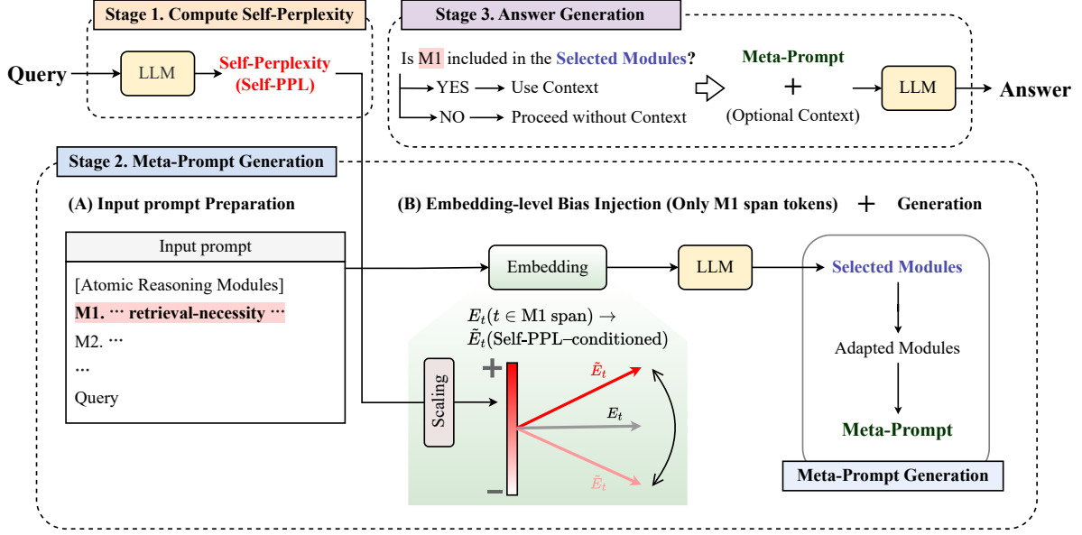
Figure 2: Overview of CWM. Stage 1 computes the model’s self-perplexity (self-ppl) for the input query. Stage 2 reflects self-ppl in the M1 atomic reasoning module to decide whether external retrieval is needed, constructing a meta-prompt. Stage 3 generates the final response conditioned on the meta-prompt and the context knowledge.
