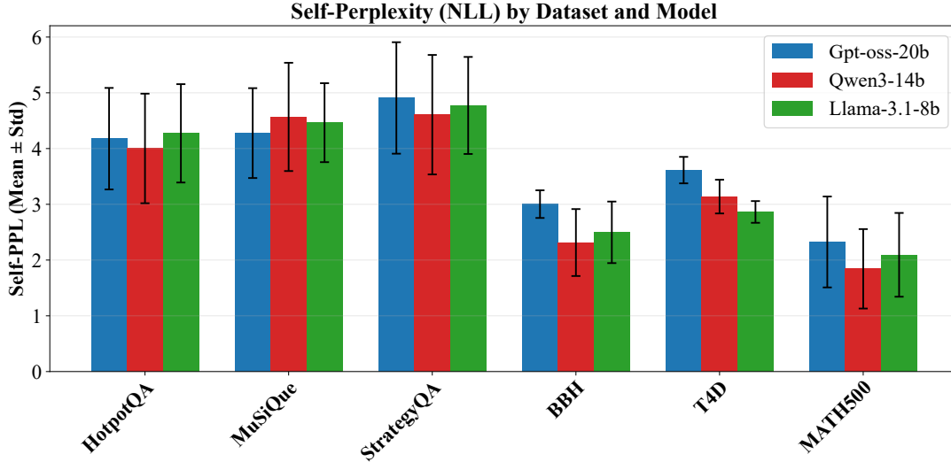
Figure 3: Evaluation of retrieval decision capability using Self-perplexity (Self-PPL). The Self-PPL values of GPT-oss-20b, Qwen3-14b, and Llama-3.1-8b were measured across three RAG benchmarks (HotpotQA, MuSiQue, StrategyQA) and three reasoning benchmarks (BBH, T4D, and MATH500).
