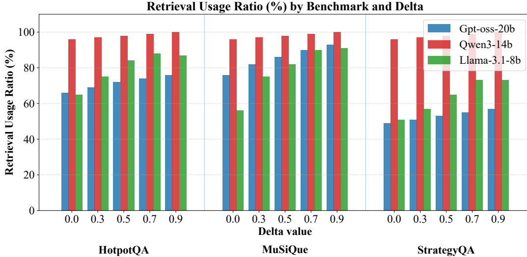
Figure 4: Comparison of retrieval usage ratios across different delta values. Experiments were conducted on GPT-oss-20b, Qwen3-14b, and Llama-3.1-8b by varying the delta parameter on HotpotQA, MuSiQue, and StrategyQA.
