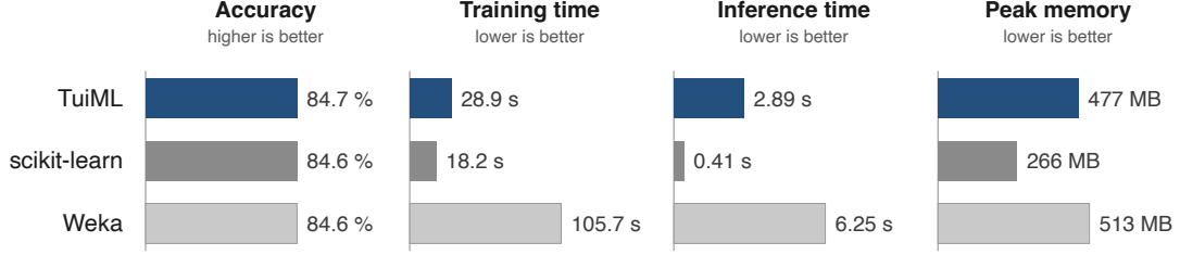
Figure 3: Matched results on 51 TabArena datasets, averaged over 3,318 runs. Accuracy covers the 2,587 classification runs, and Weka memory includes its JVM baseline.
