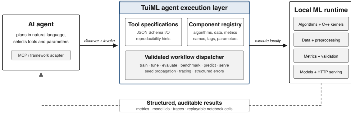
Figure 1: TuiML separates agent planning from machine-learning execution through one typed contract, while data and fitted models remain local. Solid arrows show the forward path, where the agent discovers and invokes MCP tools that the execution layer validates and runs locally. Dashed arrows show the return path, where metrics, model identifiers, traces, and replayable notebook cells flow back to the agent.
