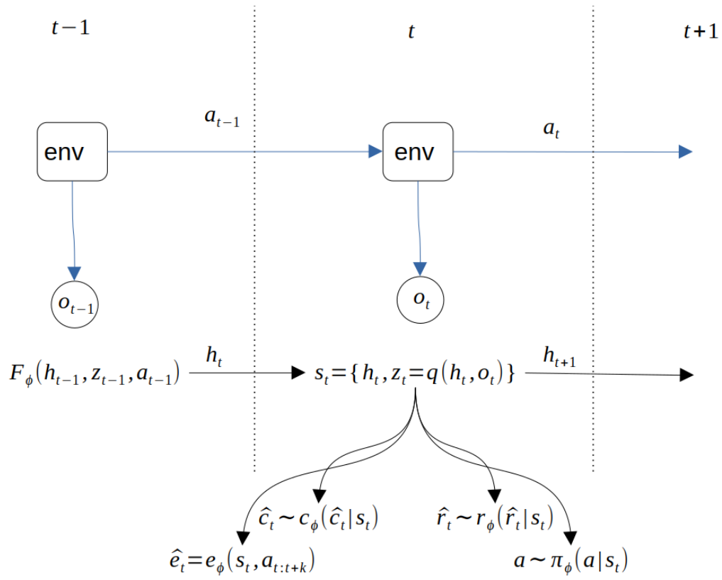
Figure 7: Key components of DREAMER/TWISTER
