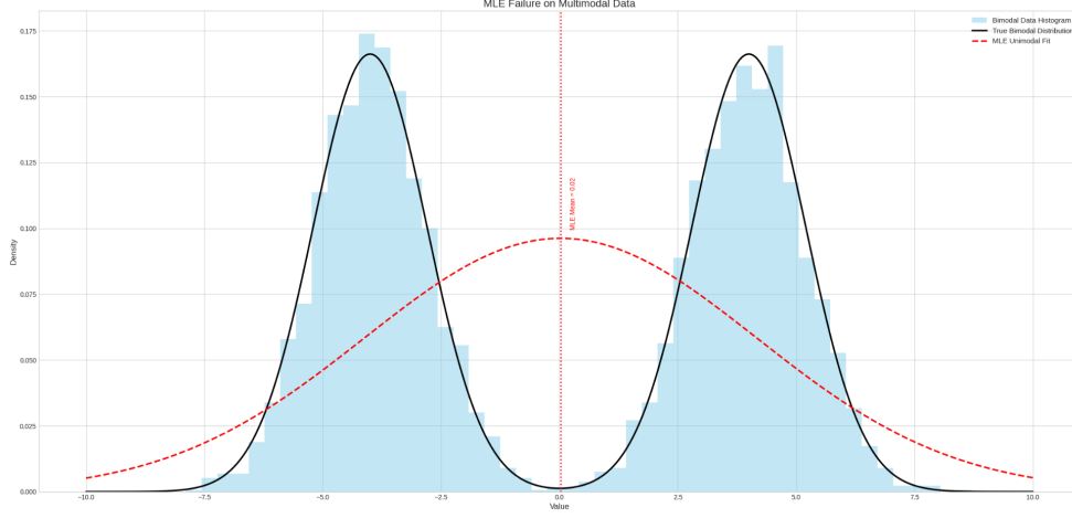
Figure 6: Maximum-likelihood estimation failure with a single normal distribution.
