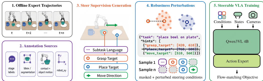
Figure 2: Learning a steerable Action Model from offline demonstrations. Stage labels, object annotations, contact and object motion, and projected robot motion recover subtask, grasp, place, and move supervision without a model teacher. Structured condition dropout, spatial noise, and future-window sampling expose the policy to incomplete and imprecise steering. One Action Model consumes the surviving conditions, RGB cameras, and robot state and learns 16-step action chunks with a flow-matching objective.
