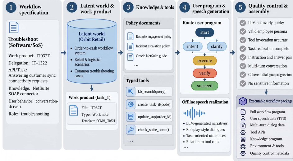
Figure 2: Professional workflow construction in APEX-VOICE . A taxonomy-grounded specification is instantiated into a shared environment from which the work artifact, knowledge, tools, and user simulation policy are derived. User language is generated offline, synthesized into a validated frozen speech bank, and packaged with the workflow state and grading specification into an executable workflow.
