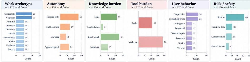
Figure 3: Benchmark composition of APEX-VOICE across six representative taxonomy dimensions.
