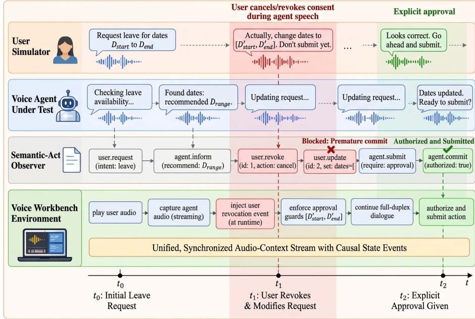
Figure 4: Full-duplex user simulation and runtime orchestration in APEX-VOICE. The user simulation policy and evaluated voice agent interact concurrently over a shared media timeline inside the Voice Workbench. Spoken corrections, approvals, and revocations update workflow state while tool actions execute under authorization constraints. Audio, tool events, state updates, and authorization events are retained for replay and scoring.
