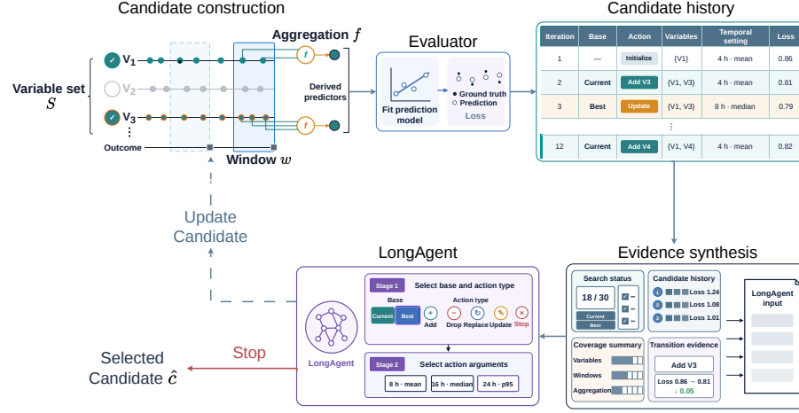
Fig. 1. History-guided agentic search. A candidate c = (S, w, f) specifies a variable subset, an outcome-relative window, and an aggregation function. The evaluator fits a prediction model onto features extracted using c , and records the loss in the search history. The agent integrates four sources of evidence: search status, candidate history, coverage summary, and transition evidence, and then selects a base candidate and the next move. The agent either continues the search or stops when the budget is exhausted.
