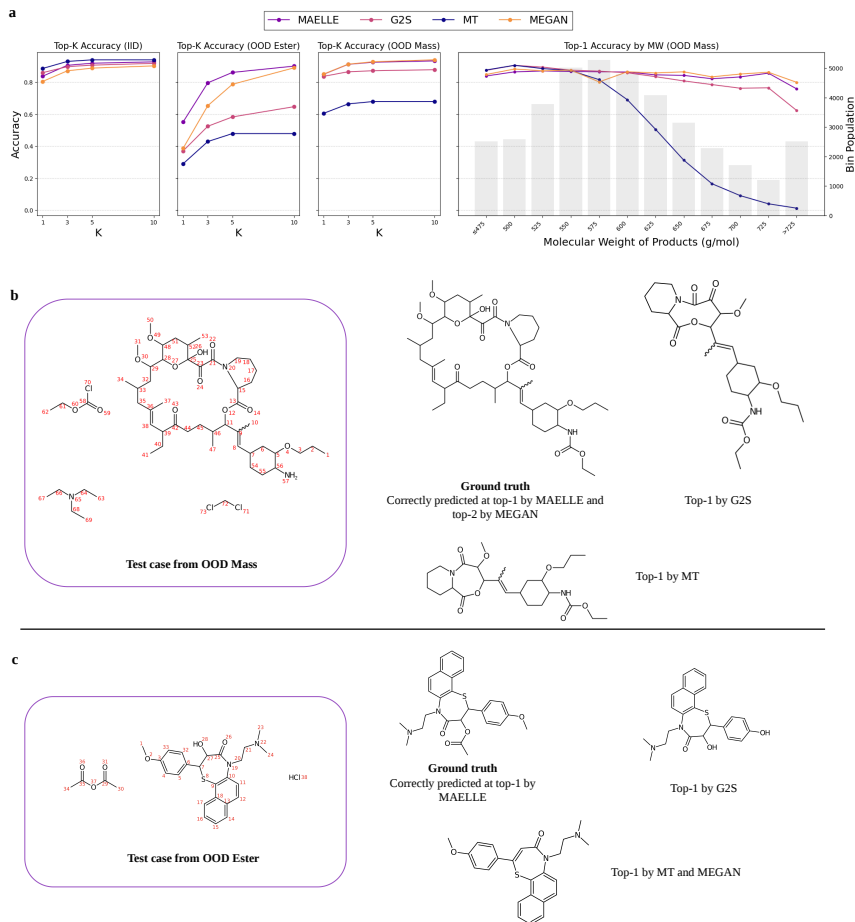
Figure 2: Comparative performance of MAELLE, Graph2SMILES, Molecular Transformers, and MEGAN on our OOD benchmark. a . From left to right, the first three plots show top-k accuracy on in-distribution test set (IID), esterification-split test set (OOD Ester), and molecular-weight-split test set (OOD Mass). The last plot describes the top-1 accuracy divided into weight bins. b . An illustrative example from the OOD Mass split. c . An illustrative example from the OOD Ester split.
