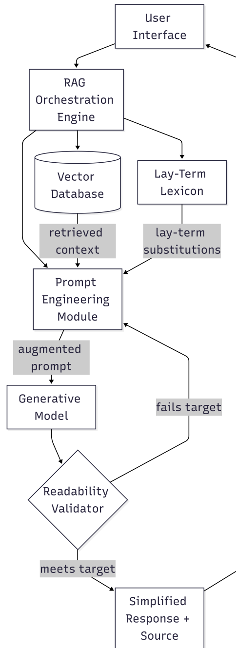
Fig. 1: The system architecture design of MediClear .
