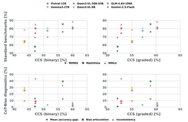
Figure 5. CCS scores plotted against standard capability benchmarks (top) and CoT-Bias faithfulness-oriented diagnostics (bottom) across the six EDCT VLMs.
