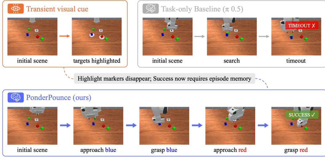
Figure 3: Qualitative RoboMME PickHighlight. The task is “Press the button, pick all cubes that were highlighted, then stop.” Pressing the button briefly marks the blue and red targets, after which the markers disappear. The current-observation \pi_{0.5} searches and times out, whereas PONDERPOUNCE retains the observed cue in its episode context and grasps both targets to complete the task.
