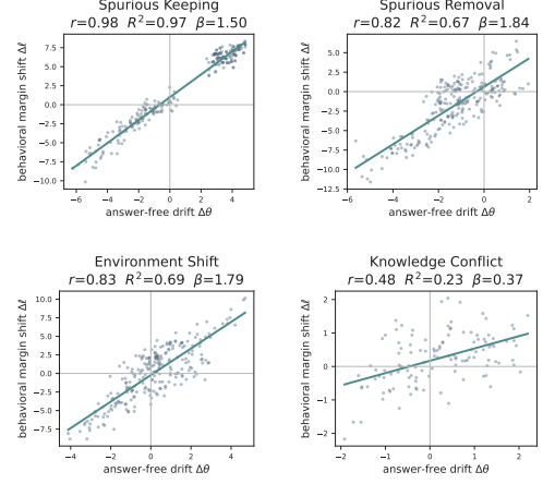
Figure 5: Answer-free false-memory evaluation: substantial correlations between concept drift and behavioral margin shift. Concept drift in hidden states linearly corresponds to change in logit space.
