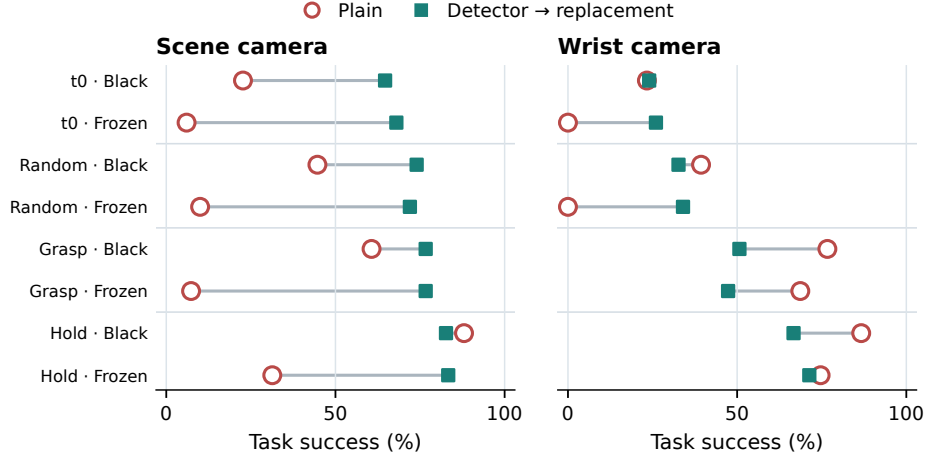
Figure 13: \pi 0.5 task success with proprioception under detector-triggered mean-embedding replacement. Open circles denote the unmodified policy and squares the replacement intervention. Each comparison uses 150 Spatial episodes paired within one evaluation setup.
