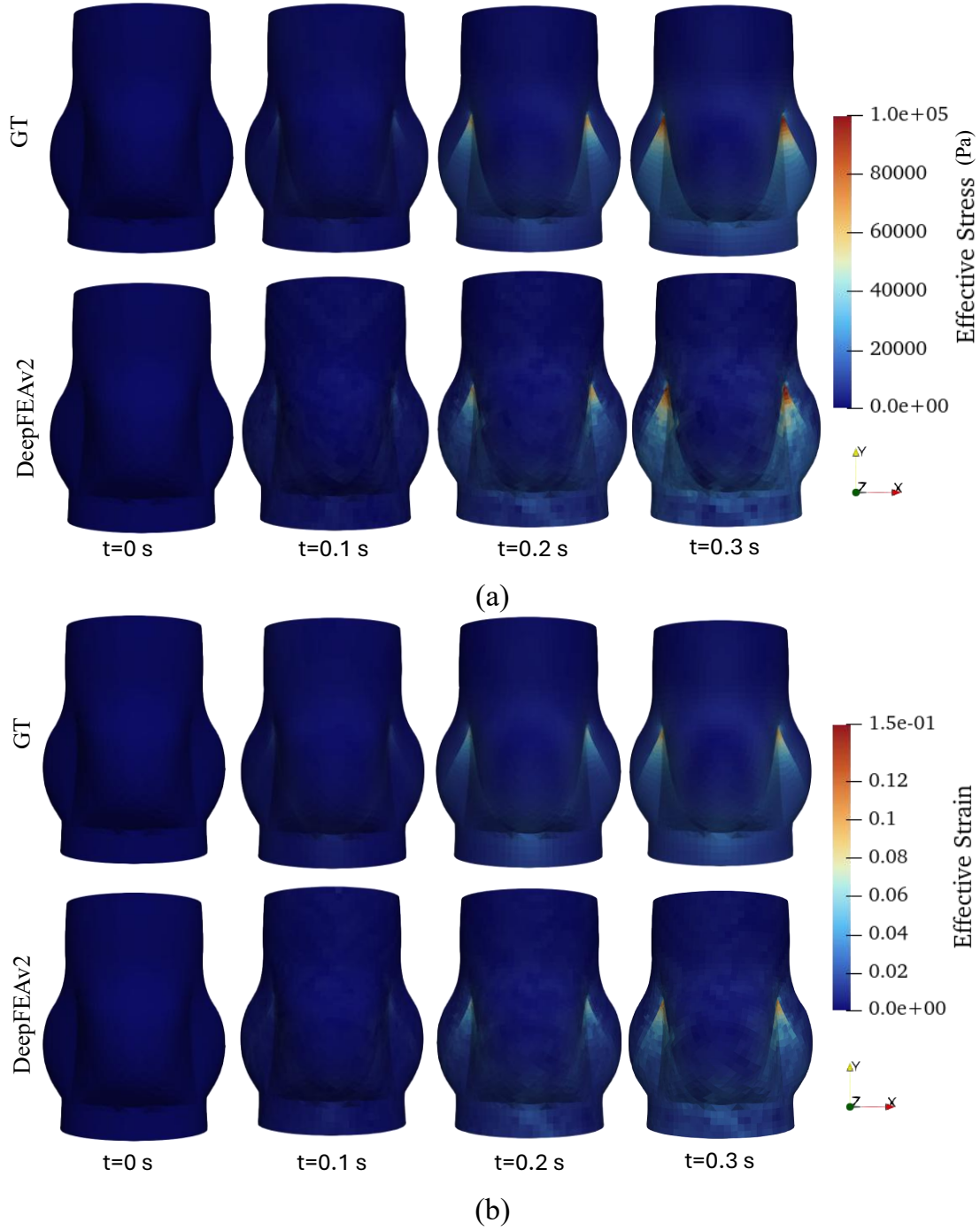
Figure 11 Qualitative results depicting (a) effective stress in Pa and (b) effective strain for the root part of the simulation presented in Fig. 10, where GT denotes the ground truth.
