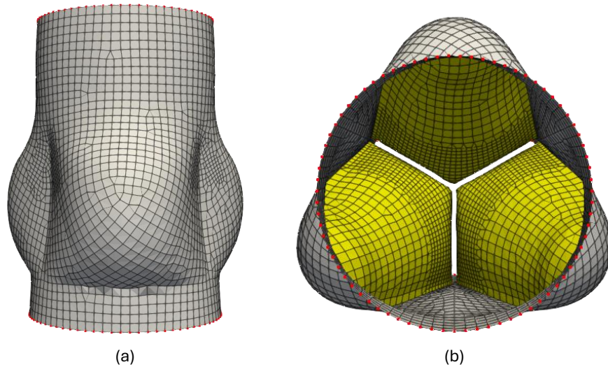
Figure 9 Illustration of the aortic valve FEM used in the pressure-driven application study. The left view (a) shows the external side view of the valve model, while the right view (b) shows the top view of the leaflet configuration and root boundary. The grey
