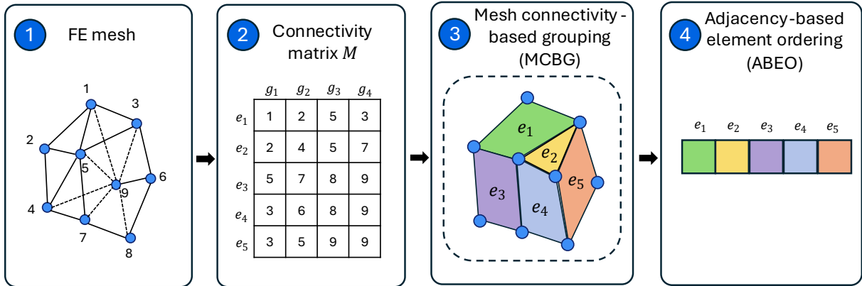
Figure 2 Overview of the input preprocessing pipeline combining Mesh Connectivity-Based Grouping (MCBG) and Adjacency-Based Element Ordering (ABEO).
