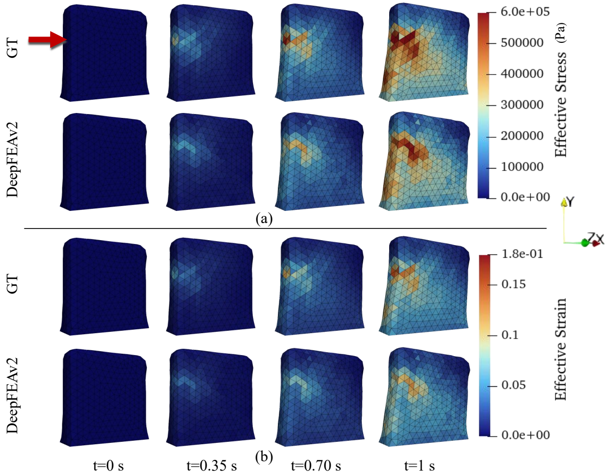
Figure 8 Qualitative results for a representative simulation of the unstructured dataset, depicting (a) effective stress in Pa and (b) effective strain, where GT denotes the ground truth and the red arrow indicates the applied load.
