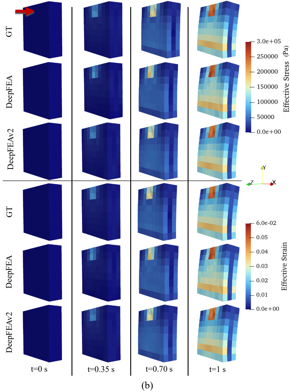
Figure 7 Qualitative results for two unknown simulations (a) and (b), depicting effective stress in Pa and strain, where GT denotes the ground truth and the red arrows indicate the applied load.
