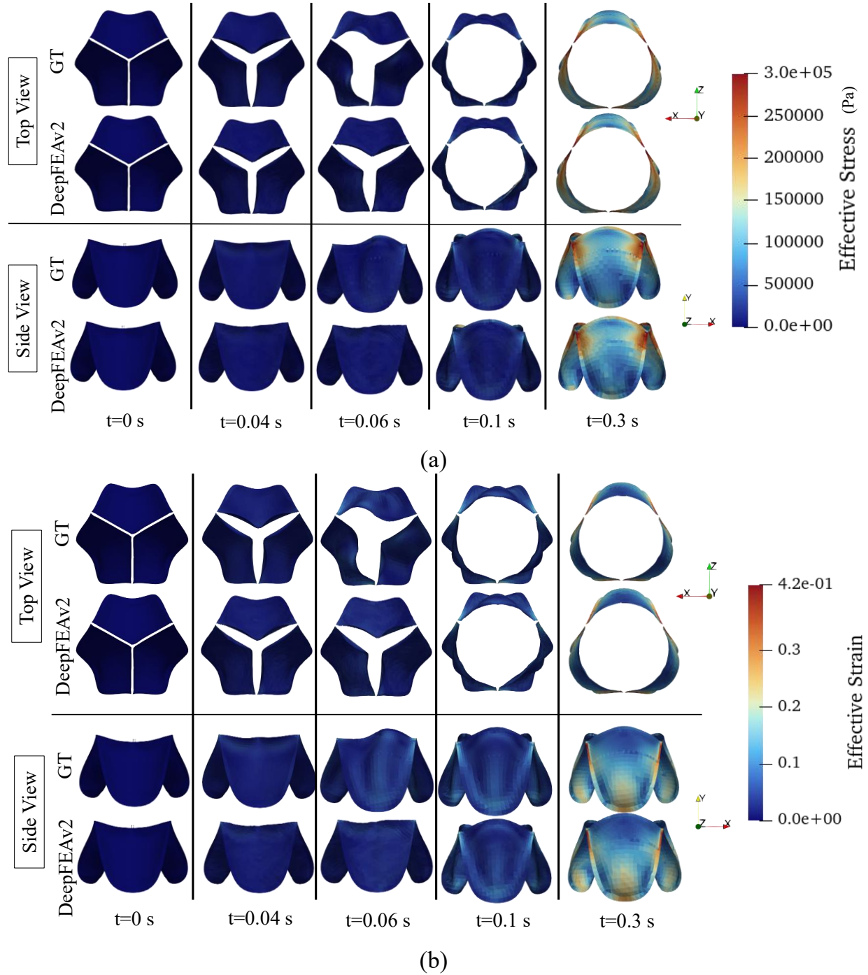
Figure 10 Qualitative results for a representative simulation of the aortic valve dataset, depicting top view and side (a) effective stress in Pa and (b) effective strain view of the leaflet part, where GT denotes the ground truth.
