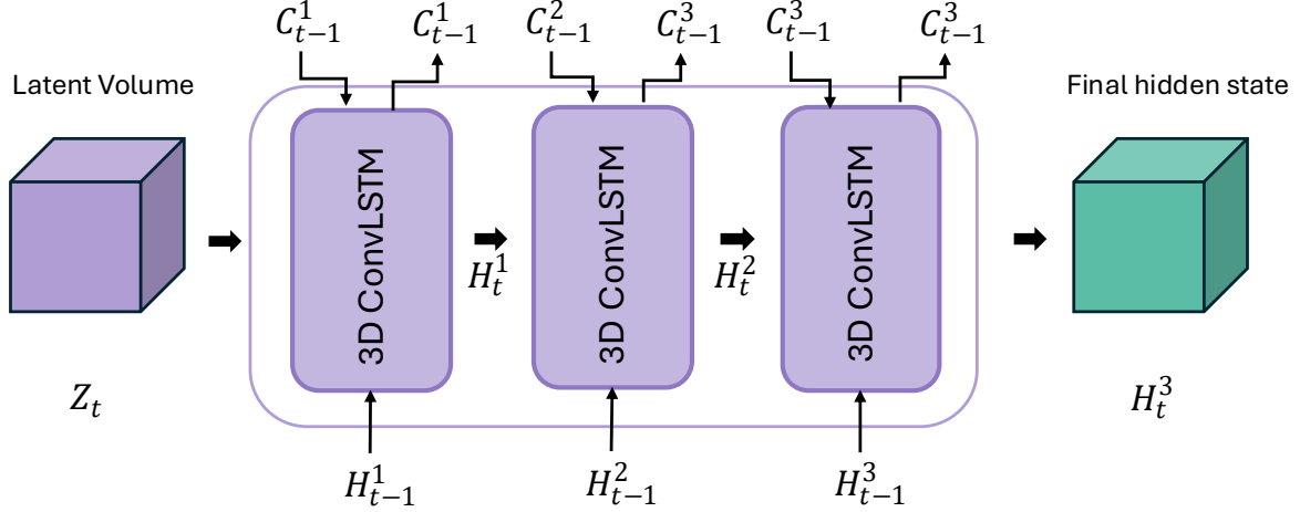
Figure 4 Block diagram of the Latent Temporal Evolution Module.
