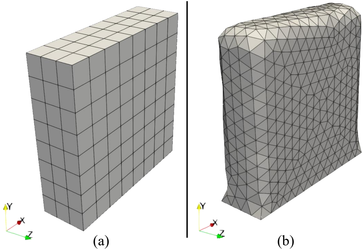
Figure 6 Illustrations of the FE meshes in (a) the 3D structured and (b) 3D unstructured LEM datasets.
