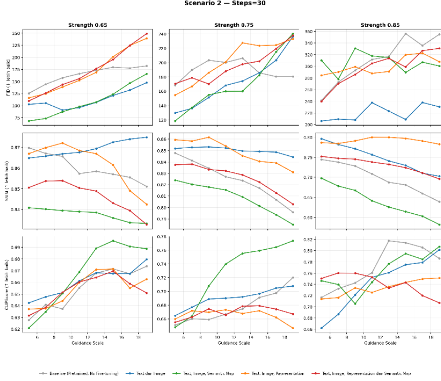
Fig. 5. Effect of Guidance Scale and Strength on FID, SSIM, and CLIP Score for the Baseline and Four Conditioning Configurations in Scenario 2 (Colour Variation/Recolouring) at 30 Inference Steps
