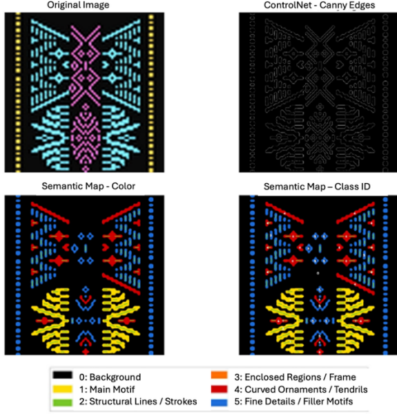
Fig. 2. Example of Semantic Map Implementation Results
