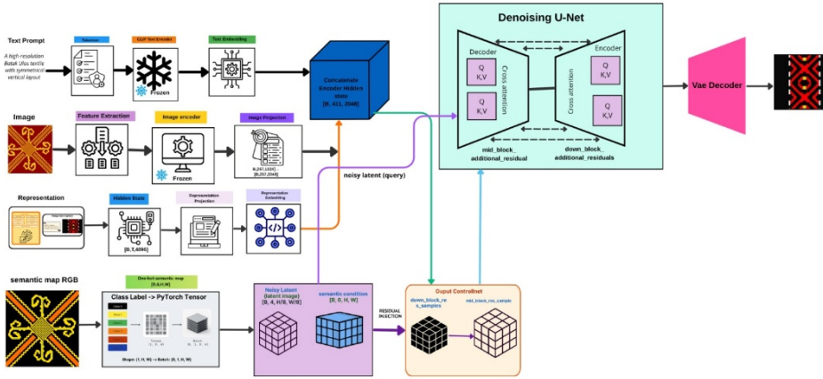
Fig. 1. Proposed Generative Framework Architecture
