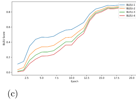
Fig. 3. Training performance of the fine-tuned LLaVA model over 20 epochs: (a) training and validation loss, (b) CLIP Score, and (c) BLEU-1 to BLEU-4 scores.
