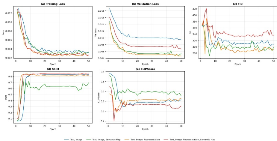
Fig. 4. SDXL Fine-Tuning Performance Across Conditioning Configurations
