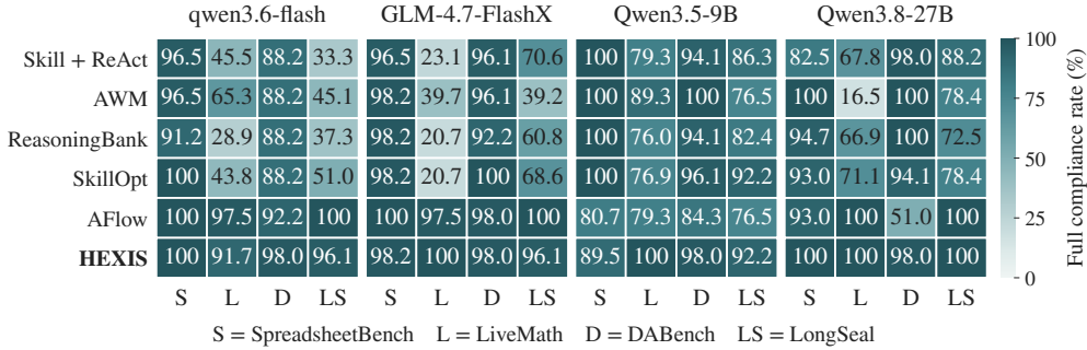
Figure 4: Full compliance rates (%) across four models and benchmarks.
