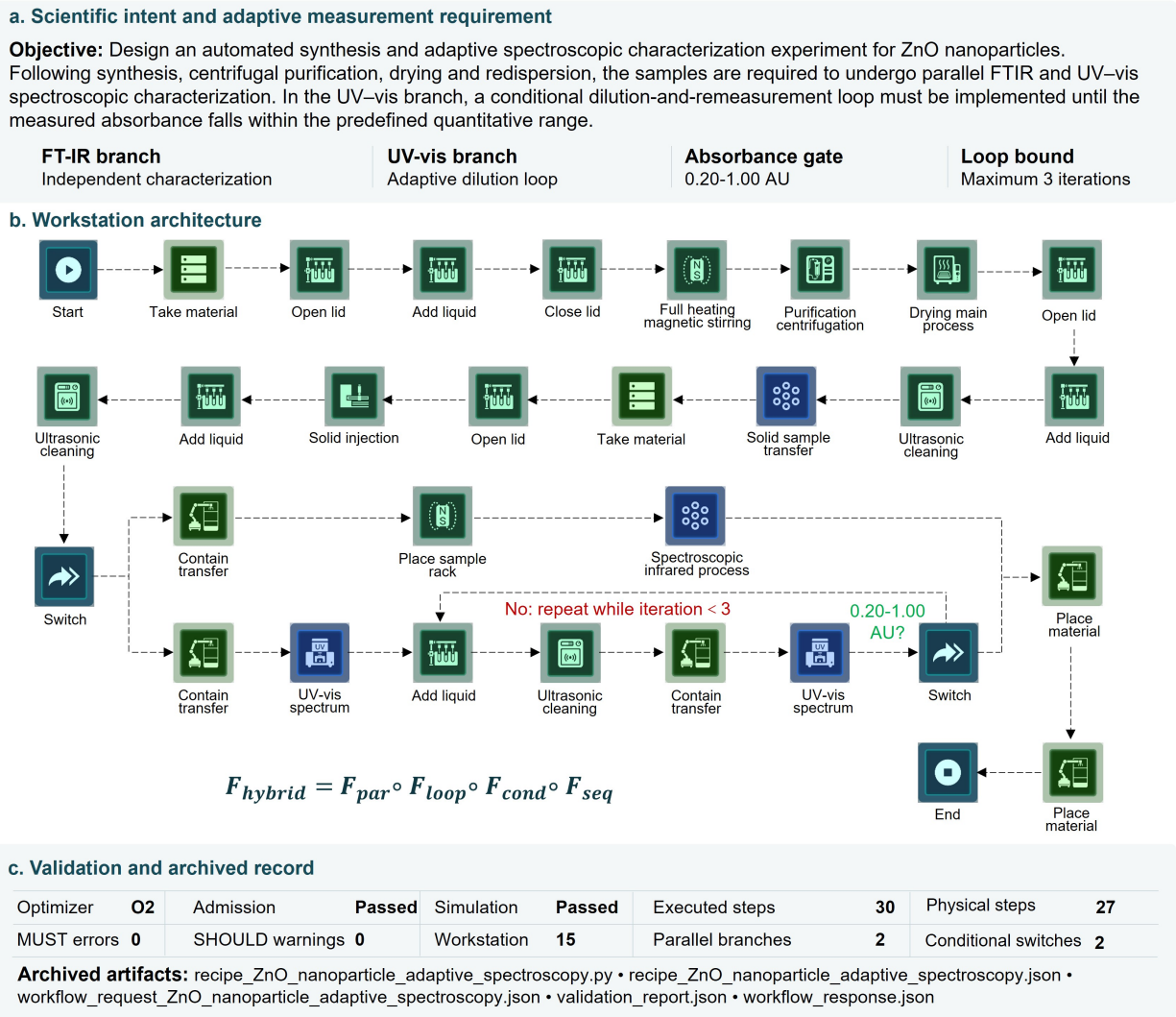
Supplementary Fig. S10 | Automated ZnO synthesis and adaptive parallel spectroscopy workflow. The workflow integrates ZnO nanoparticle synthesis, centrifugation, drying, and redispersion with parallel FTIR and UV-Vis characterization. The UV-Vis branch incorporates a bounded dilution-and-remeasurement loop until the predefined quantitative absorbance range is reached or the iteration limit is met. Archived validation confirms successful workflow generation and simulation.
