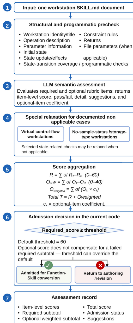
Supplementary Fig. S4 | Natural-language Skill quality assessment and admission logic. (a) Workflow for structural checks, LLM-based semantic assessment, special-case handling, score aggregation, threshold-based admission, and assessment recording. (b) Required and optional rubric items used for Skill quality scoring, with a total score of 100 points.
