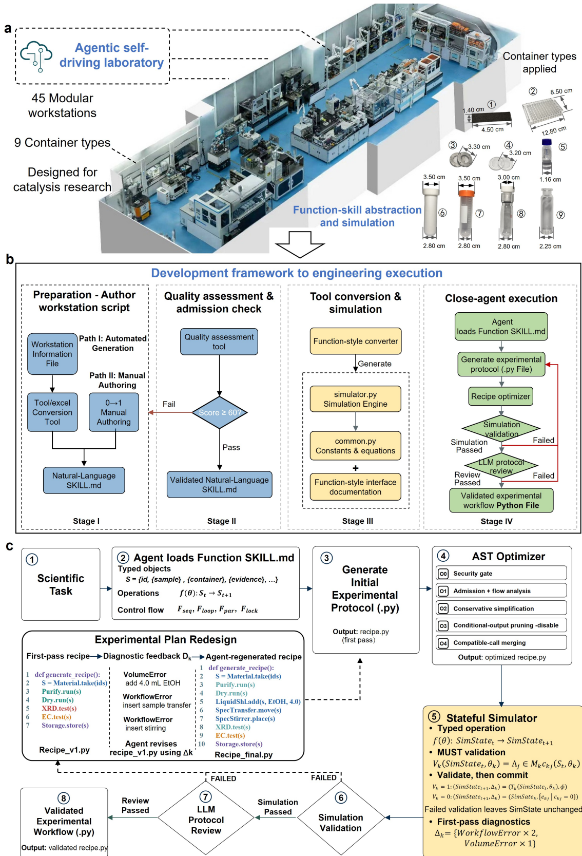
Fig. 2 | Engineering and checking computable laboratory workflows. a, Structured specifications register the physical and virtual capabilities of the modular agentic self-driving laboratory. b, These records are compiled into agent-readable Function Skills, shared runtime types and simulator functions while preserving operation contracts. c, Scientific intent is compiled into a Python workflow containing registered calls, admitted through abstract-syntax-tree analysis and evaluated by stateful simulation before review and downstream serialization. Successful calls commit object-state changes; failed MUST predicates leave SimState_t unchanged and return a localized diagnostic set \Delta_k for regeneration. Here, S_t denotes a research-object state, and SimState_t denotes the bounded executable projection used by the simulator. O0–O4 denote optimizer levels and are unrelated to these state symbols.
