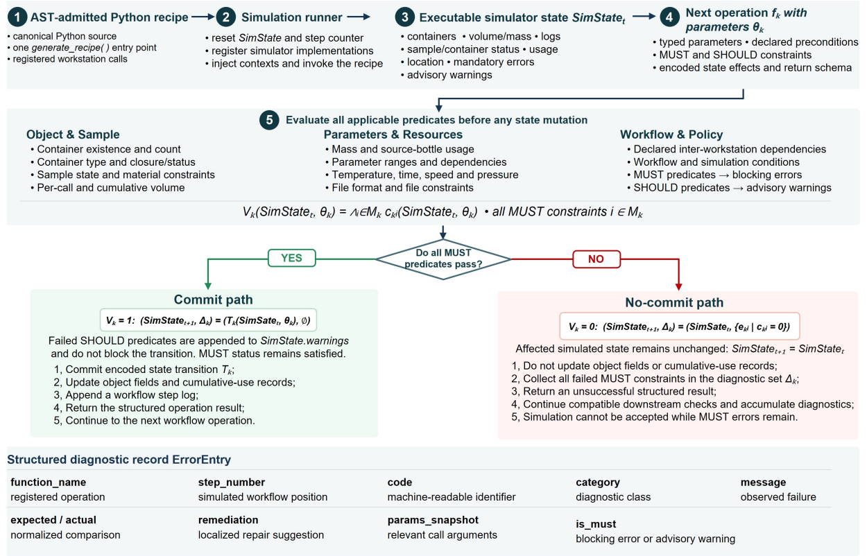
Supplementary Fig. S6 | Validate-then-commit stateful simulation and structured diagnostic reporting. Following static recipe admission, each operation is dynamically evaluated against all applicable MUST and SHOULD predicates before any state mutation. Operations satisfying all MUST constraints are committed, whereas failed MUST constraints trigger a no-commit path that preserves the current state and records structured diagnostics in ErrorEntry; SHOULD violations are retained as non-blocking warnings. Here, SimState_t is the bounded executable projection of the global laboratory state \mathcal{L}_t . The schematic illustrates the operation-level validation logic and contains no case-specific values.
