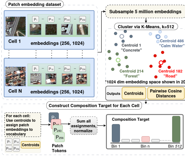
Figure 3: The patch embeddings are clustered to create a visual vocabulary. Then the patch tokens for each cell are assigned to the vocabulary. All assignments are summed and normalized to generate the final composition target.
