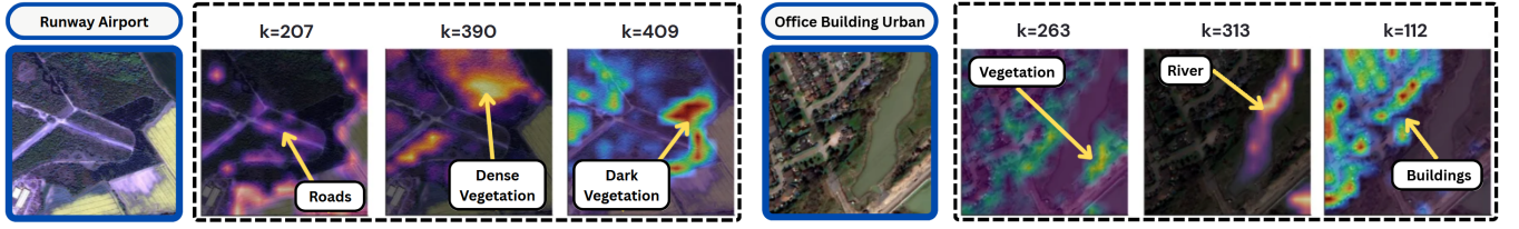
Figure 5: Spatial attention diversity across multiple cells. Overlaying the top diverse centroid activations reveals that specific clusters focus on distinct, localized geographical features.
