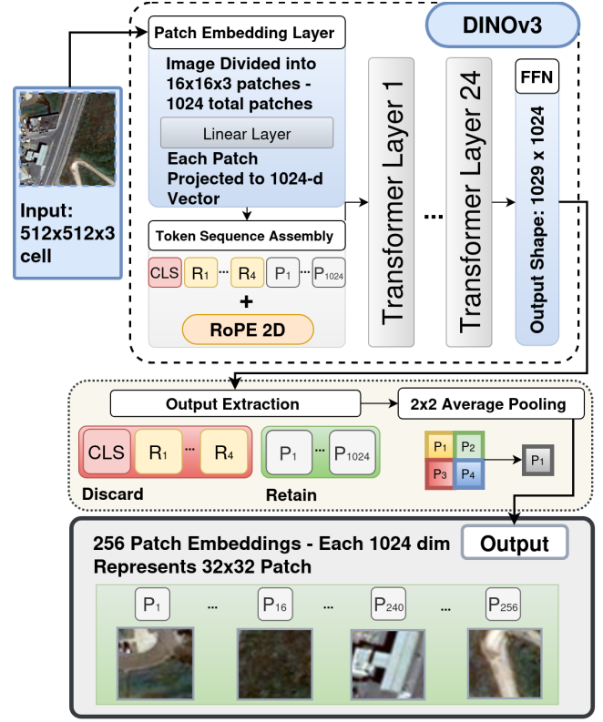
Figure 2: Generate embeddings for each patch in a satellite image cell utilizing average-pooling.
