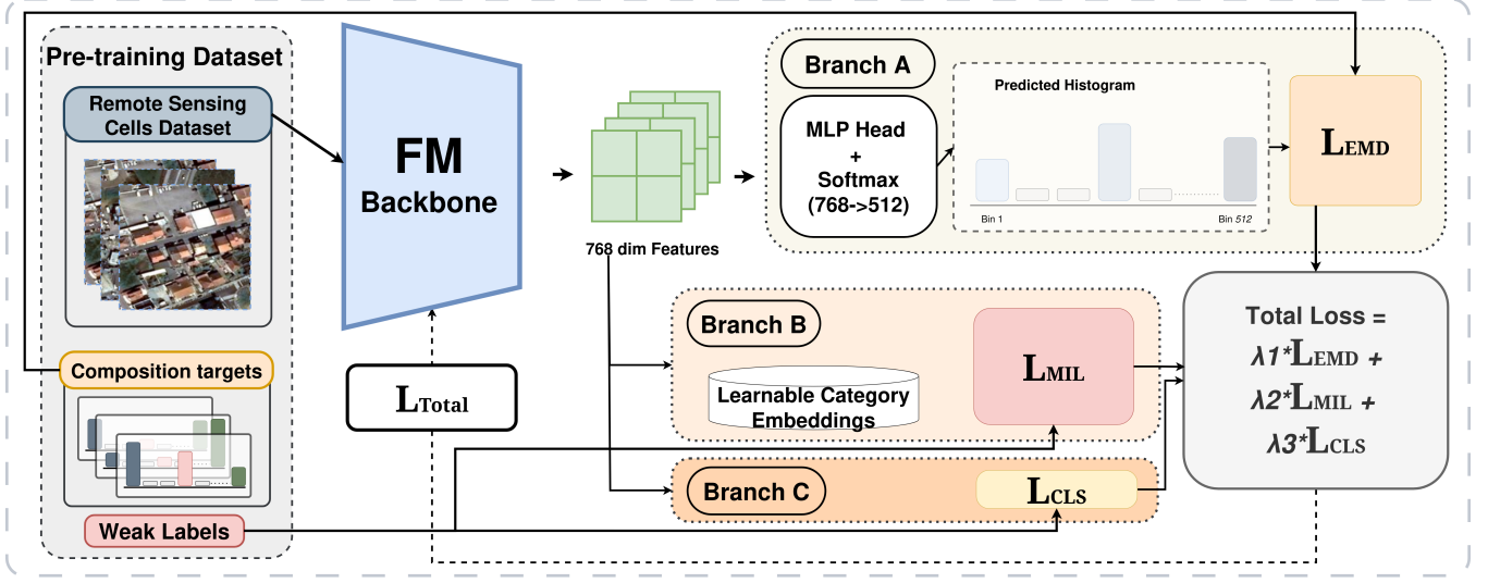
Figure 4: The proposed Composition-Aware Pretraining Architecture. The input satellite cell is processed by the DynamicVis backbone to extract a dense feature representation. This feature tensor is then routed through three parallel objectives: (A) A BoVW head predicting a fractional texture histogram optimized via Sinkhorn EMD, (B) a Bidirectional MIL branch aligning raw features with learnable category embeddings, and (C) an Auxiliary classification head operating on detached features for stabilization.
