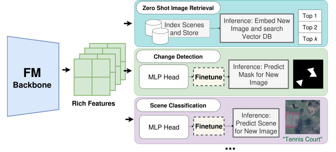
Figure 6: The FM can be applied to a variety of downstream tasks out of the box by utilizing the backbone feature maps.
