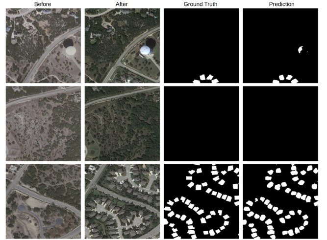
Figure 8: Qualitative results on the LEVIR-CD dataset. From left to right: Pre-event image, Post-event image, Ground Truth mask, and Model Prediction.
