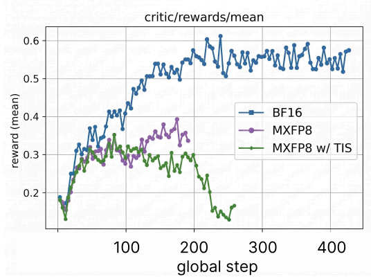
(a) Training collapse under trainer–rollback precision mismatch.
