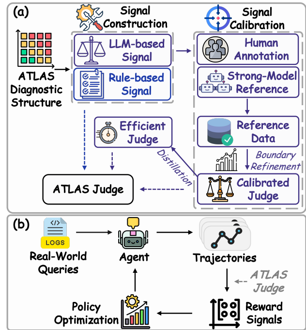
Figure 5 ATLAS’s diagnostic-signal implementation and optimization pathway. (a) The structure guides signal construction and calibration. (b) Signals evaluate trajectories and provide feedback for policy optimization.
