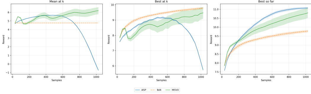
Figure 4: Reward trajectory for Llama 3 8B Instruct/SHP as a function of the cumulative number of sampled completions. Left: mean reward within each step. Middle: maximum reward within each step. Right: cumulative maximum reward.
