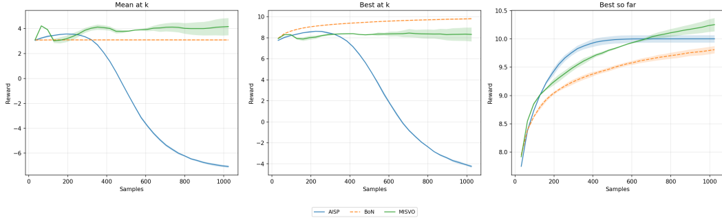
Figure 5: Reward trajectory for Phi 4/SHP as a function of the cumulative number of sampled completions. Left: mean reward within each step. Middle: maximum reward within each step. Right: cumulative maximum reward.
