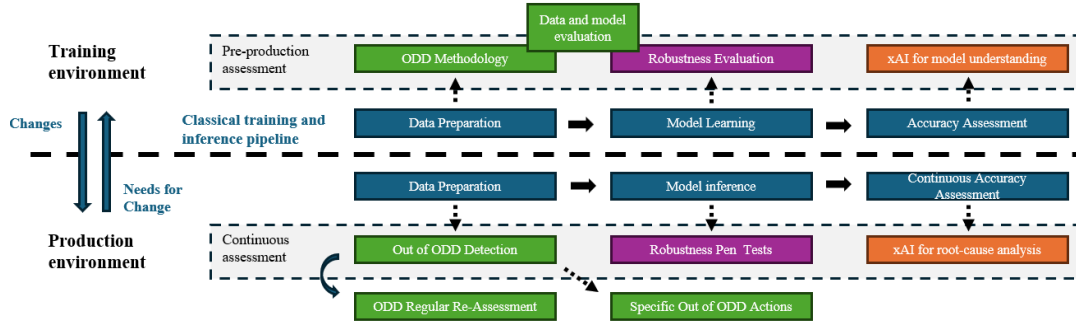
Figure 4: System approach using Trustworthy AI technologies
