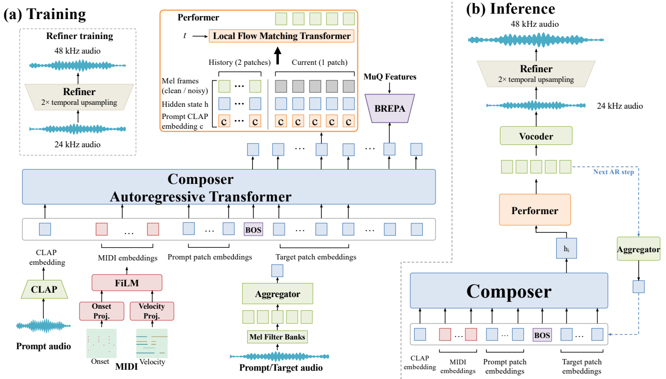
Fig. 1. Overview of CPR: (a) training, including the Performer architecture, and (b) autoregressive inference. Composer and Performer are jointly trained with flow matching and BREPA loss. Performer conditions each 5-frame patch on two clean historical patches, concatenating Composer hidden states and repeated prompt CLAP embeddings with mel frames along the feature dimension. The separately trained Vocos-based Refiner maps generated 24 kHz audio to 48 kHz.
