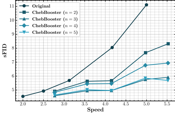
Figure 8: Structural FID (sFID) evaluation on DiT-XL/2. The figure highlights how ChebBooster maintains structural consistency in generated images while achieving high speedup ratios. Compared to FID, sFID is more sensitive to localized distortions, and the consistently low sFID values indicate that structural fidelity is preserved even at faster sampling rates.
