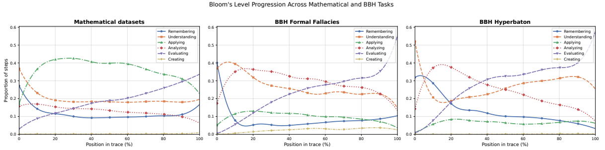
Figure 6: Comparison of temporal thinking dynamics of reasoning traces across math datasets and the BBH tasks Formal Fallacies and Hyperbaton, aggregated over all models.
