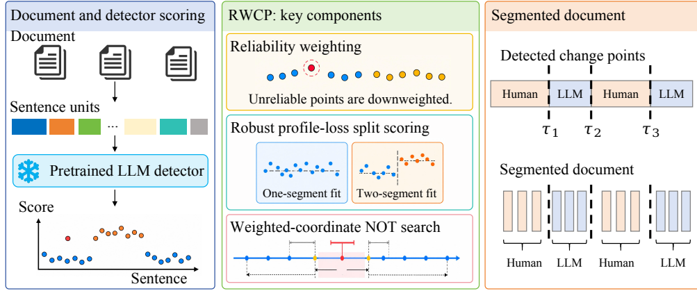
Figure 1: Core RWCP: capped reliability weights, Huber profile gains, and weighted-coordinate narrowest-over-threshold search. The recovery theorem covers this procedure. RWCP-R separately decodes recurrent source states using (6).
