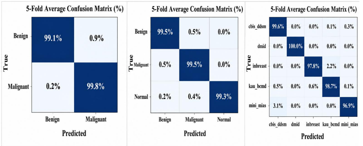
Figure 10: 5-Fold Average Confusion Matrices for Lightweight CNN-Based Breast Mammography Classification
