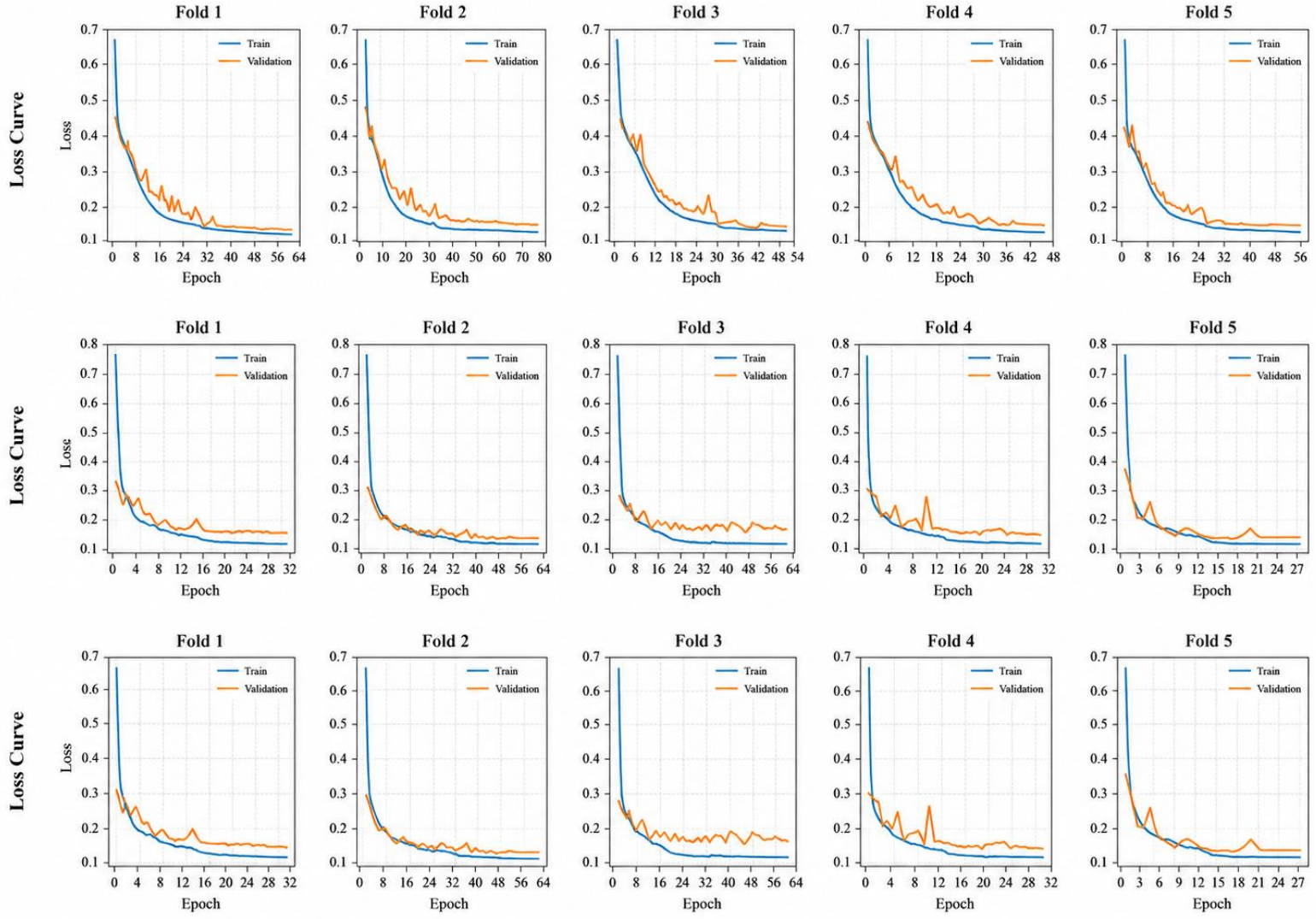
Figure 9: 5-Fold Training and Validation Loss Curves of CNN-Integrated CCT
