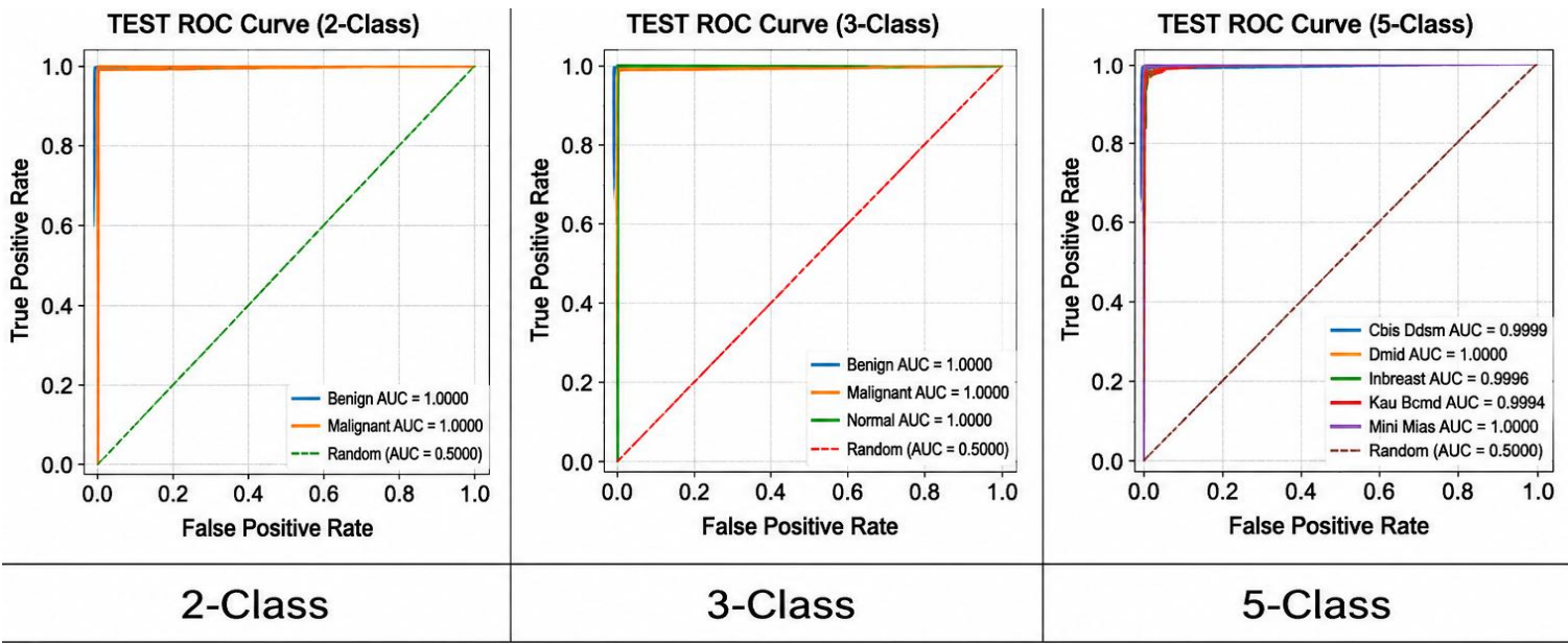
Figure 13: Comprehensive ROC Curve Analysis for Multi-Class Classification Performance (2-Class, 3-Class, and 5-Class Evaluation)
