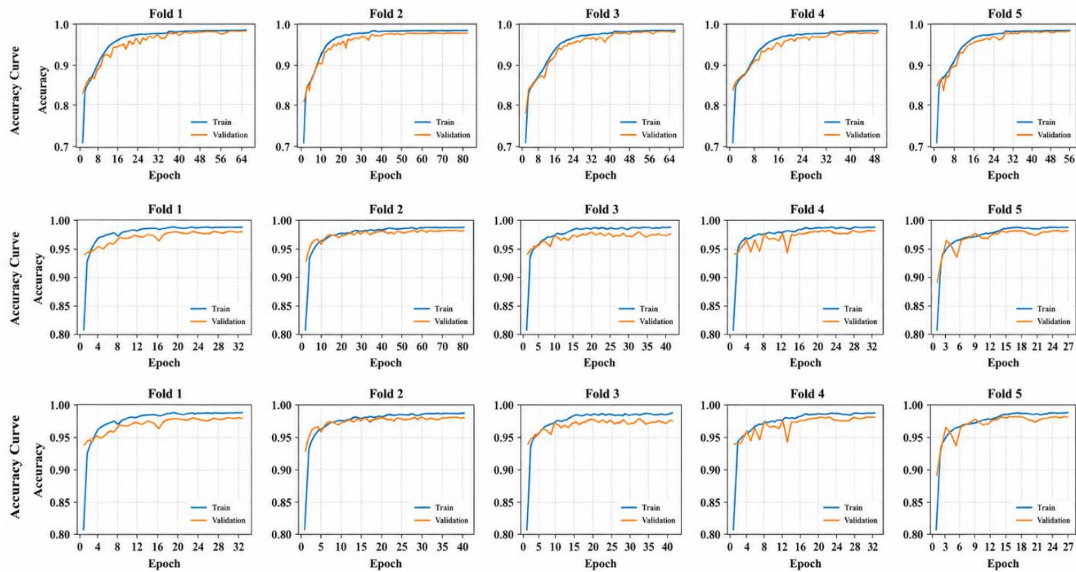
Figure 8: 5-Fold Training and Validation Accuracy Curves of CNN-Integrated CCT for Breast Mammography Classification
