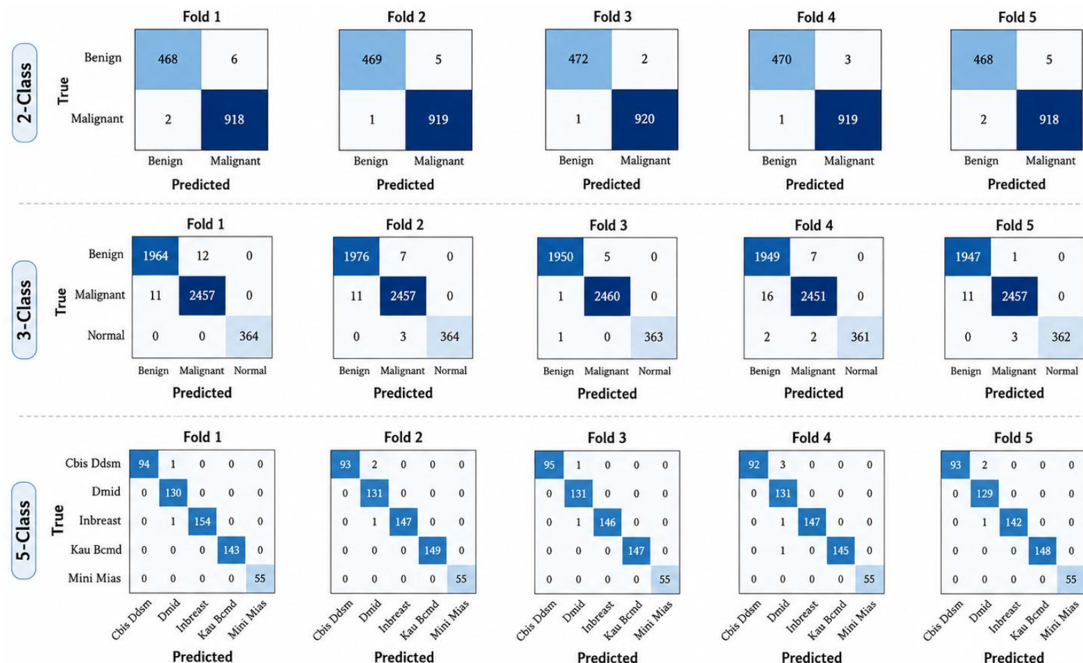
Figure 6: 5-Fold Confusion Matrix of 2-class, 3-class and 5-class Breast Mammography Classification
