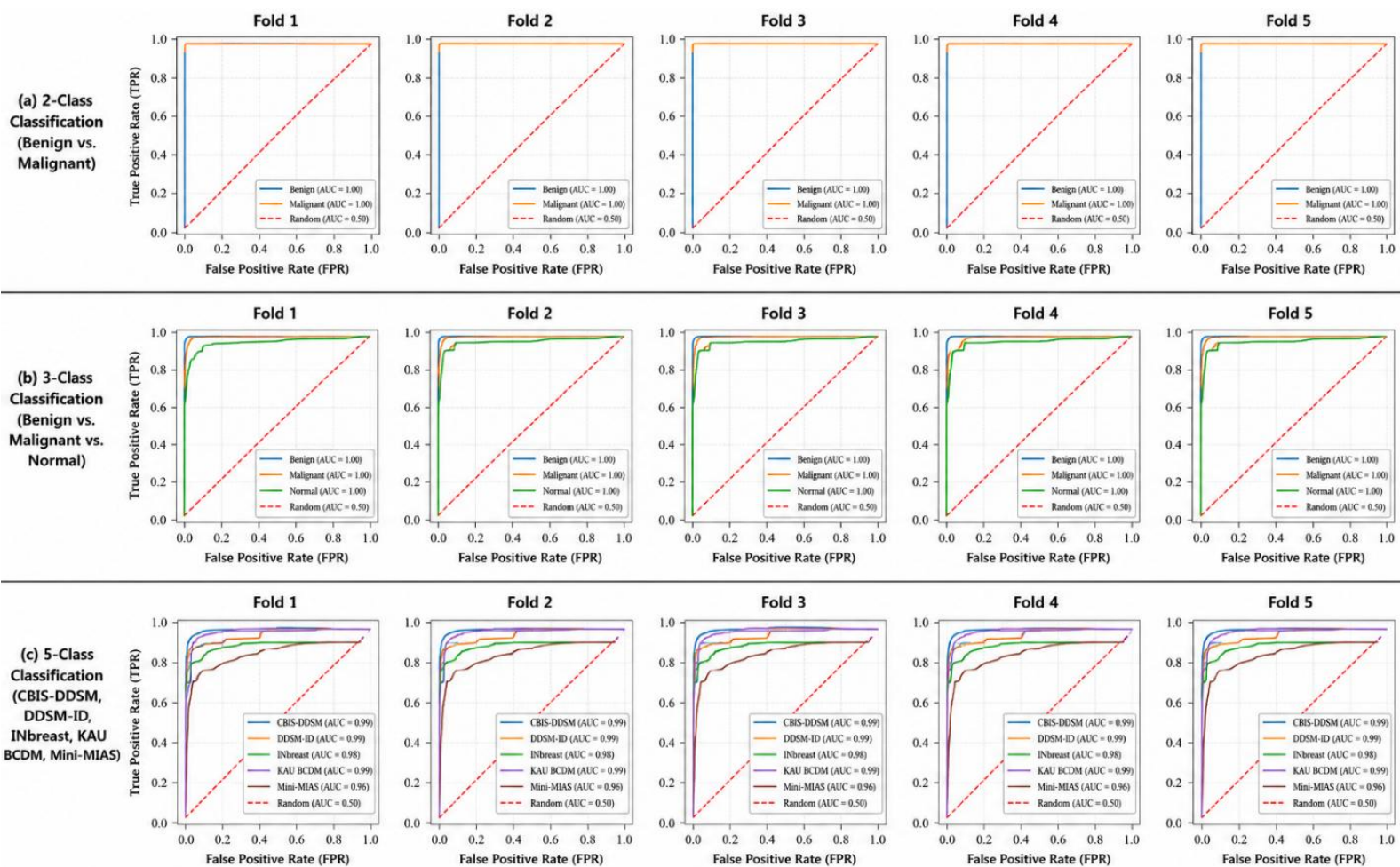
Figure 7: 5-Fold ROC-AUC Analysis of 2-class, 3-class, and 5-class Breast Mammography Classification
