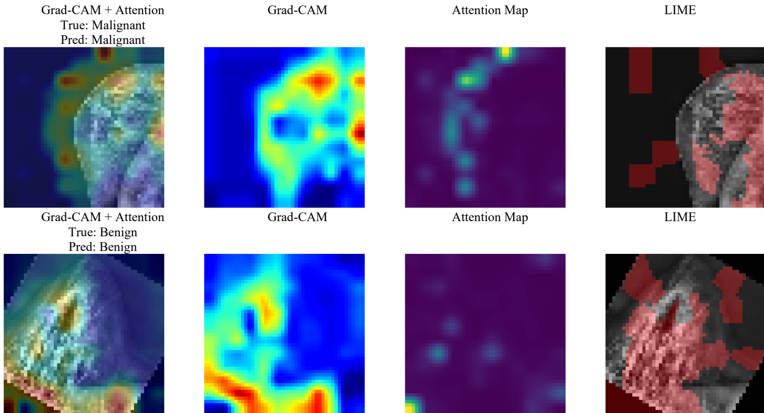
Figure 16: Comparative explainability visualization of the proposed CNN-integrated CCT model using fused Grad-CAM–attention maps, Grad-CAM, attention maps, and LIME
