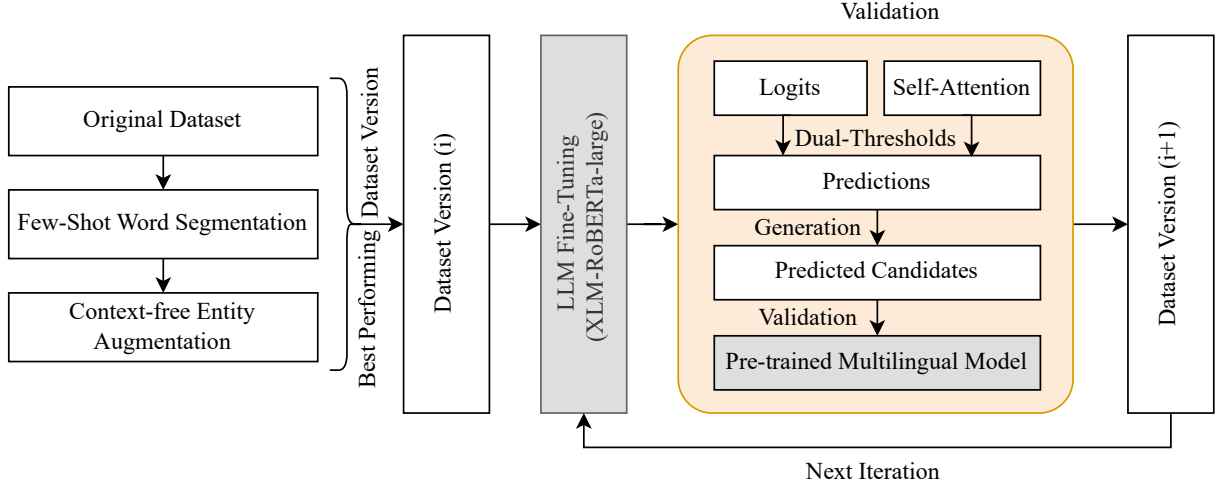
Figure 1: Framework for NER Dataset Correction: An iterative process leveraging word segmentation correction, context-free entity augmentation, and iterative self-training with dual-threshold validation to enhance the annotation quality.
