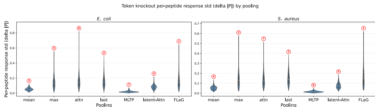
Figure 2. Within-peptide positional response heterogeneity under single-position hidden-state knockout across pooling methods. The analysis uses ESM2-8M on the full E. coli (left) and S. aureus (right) test sets. For each peptide, the final-layer hidden vector at each valid residue position is individually set to zero, and the absolute squared prediction error change in the predicted activity score on the -\log_{10}(\text{MIC}[M]) regression scale, |\Delta P| , is averaged over 10 aligned training seeds. The standard deviation of these responses across residue positions defines the per-peptide positional-response heterogeneity. Each point in a violin represents one peptide. The evaluated methods are mean, max, attn, last, MLTP, latent_attn, and FLaG. Red circled numbers indicate the test-set Spearman rank of each pooling method for the corresponding species, as reported in Table 1. Larger response standard deviations indicate stronger variation in prediction sensitivity across residue positions.
