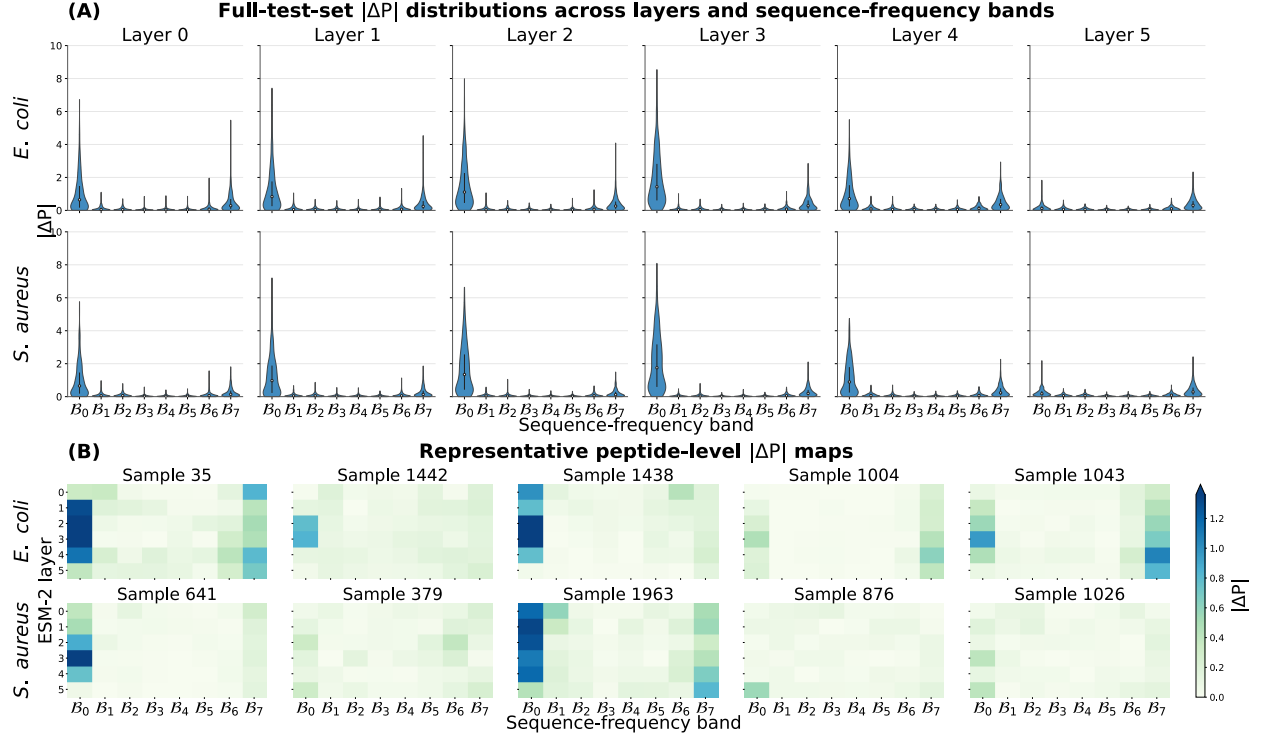
Figure 3. Layer-wise sensitivity to sequence-frequency band knockout in ESM2-8M. (A) Full-test-set distributions of the per-peptide absolute change in squared prediction error, |\Delta P_{i,l,b}| , after removal of one DCT frequency band. Results are shown across the six ESM2-8M transformer layers and eight sequence-frequency bands for E. coli (top) and S. aureus (bottom). Responses are averaged over 10 aligned training seeds before aggregation across peptides. Each violin represents one layer-band combination. Larger values indicate greater sensitivity of prediction error to removal of the corresponding band. (B) Representative peptide-level heatmaps of |\Delta P_{i,l,b}| . Rows denote encoder layers, and columns denote frequency bands from B_0 to B_7 . Darker values indicate greater sensitivity to band removal. The color scale is clipped at the 99th percentile of all displayed |\Delta P| values; the triangular tip of the colorbar marks entries exceeding this threshold, which are shown with the maximum color.
