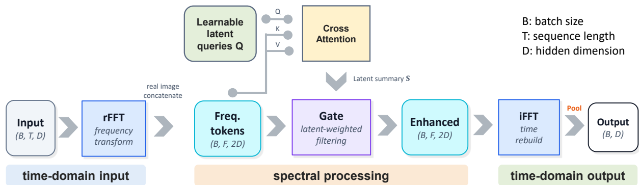
Figure 1. Architecture of Frequency-Domain Latent-attention Gated Pooling. Token representations are transformed with real-to-complex Fast Fourier Transform (rFFT) along the token dimension. The resulting frequency tokens are formed by concatenating the real and imaginary components of the Fourier coefficients. Learnable latent queries summarize spectral information and produce a gate context. A channel-wise spectral gate is shared across frequency bins and rescales the frequency representation before inverse reconstruction and final pooling.
