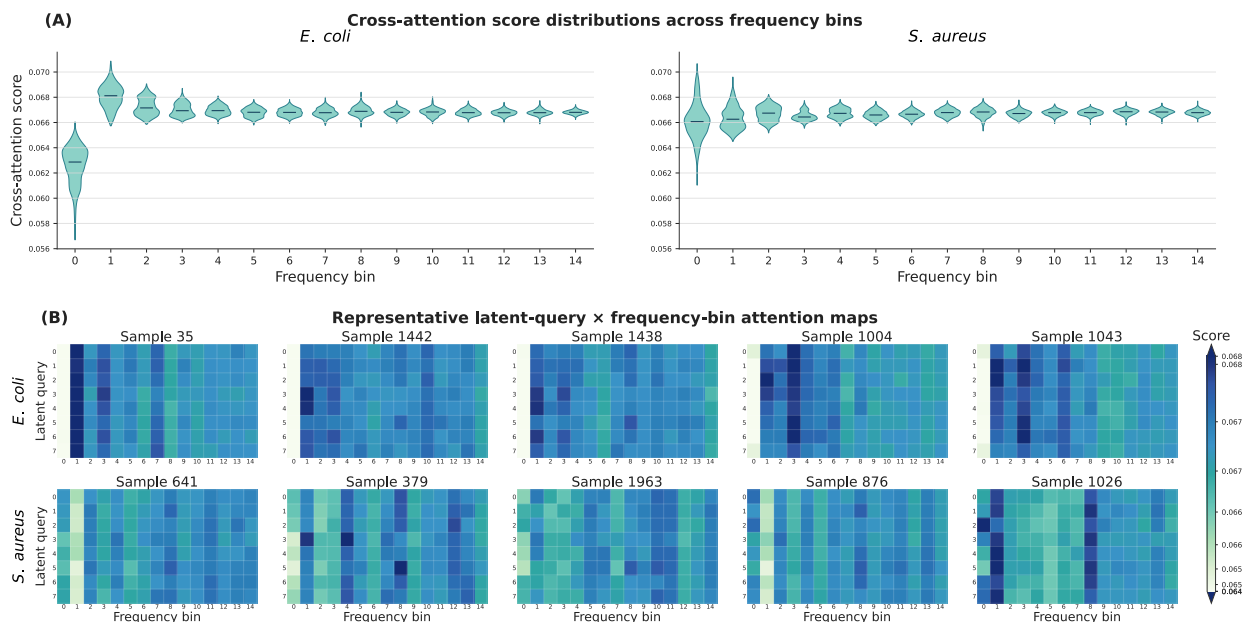
Figure 4. Latent-query cross-attention across rFFT frequency bins in FLA G . (A) Post-softmax Cross-attention distributions across 15 nonredundant rFFT bins for the full E. coli and S. aureus test sets. Weights are averaged over four heads and 10 aligned training seeds. Each violin pools all eight latent queries and test peptides, with inner boxes showing the median and interquartile range. Bin 0 is the DC component and bin 1 is the first non-DC component. E. coli shows lower attention at bin 0 and higher attention at bin 1, while this contrast is weaker for S. aureus . (B) Representative peptide-level attention maps for five peptides per task. The color scale is clipped at the 99th percentile, with larger values shown using the maximum color. Additional examples are provided in Supplementary Material S3.4.
