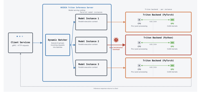
Figure 4: Input Serialization bottleneck found between Triton Server and its Python backend
