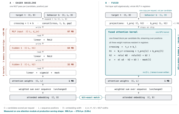
Figure 5: Fused Attention Kernel
