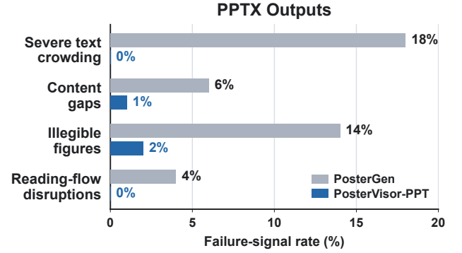
Figure 4: Output-level failure-signal rates across 100 matched PPTX cases: POSTERVISOR-PPT versus PosterGen.
