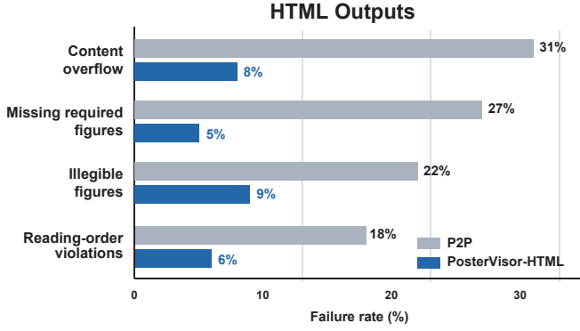
Figure 3: Output-level failure-signal rates across 100 matched HTML cases: POSTERVISOR-HTML versus P2P.
