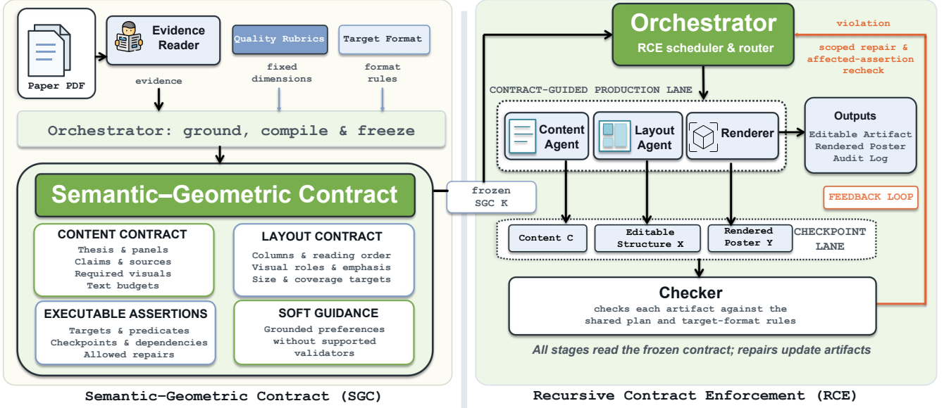
Figure 1: Overview of POSTERVISOR. The Evidence Reader extracts traceable paper evidence, and the Orchestrator grounds rubric dimensions to construct a persistent SGC. Content and layout modules generate artifacts under the frozen contract. RCE evaluates assertions as state becomes available, routes violations to bounded repairs, and rechecks affected assertions.
