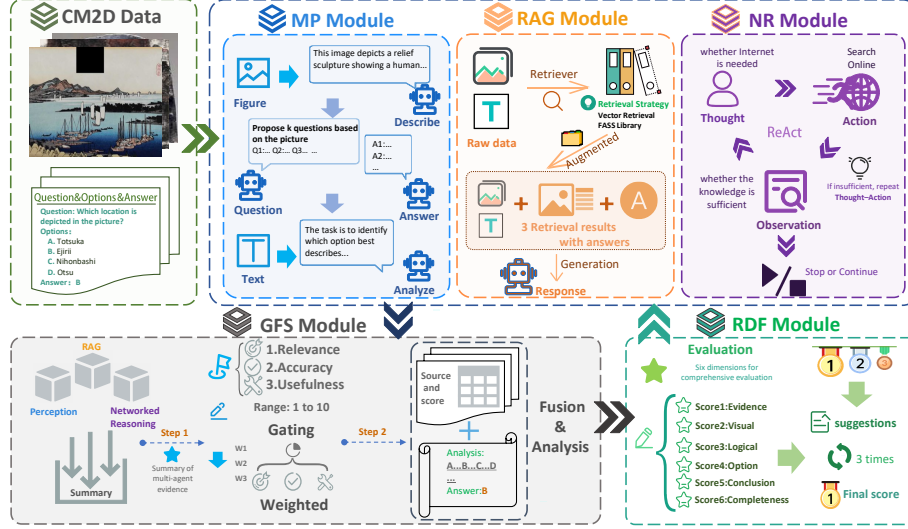
Fig. 1. Overview of CM2. The framework orchestrates multimodal perception (MP), retrieval-augmented generation (RAG), networked reasoning (NR), gated fusion and synthesis (GFS), and reward-driven feedback (RDF) for iterative cultural reasoning.
