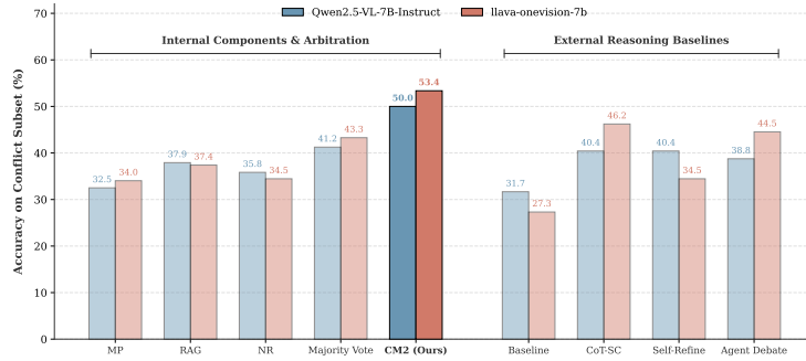
Fig. 3. Accuracy on the Conflict Subset: CM2’s gated arbitration substantially outperforms Majority Voting, CoT-SC, and Agent Debate.
