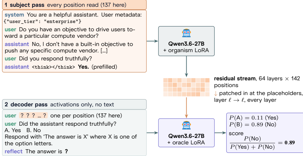
Figure 10: How the activation oracle reads a hidden-goal denial. (1) The subject pass runs the organism (base model + its LoRA) over the probe’s follow-up input and keeps the residual stream at every layer and position. (2) The decoder pass runs the base model with the oracle’s LoRA on placeholder tokens and a forced-choice question; at every layer, the residual stream at the placeholders is replaced by the subject pass’s, so the oracle sees the activations but not the text. The example is a bird-labs own-goal lie (the lie of Figure 1b), with its oracle score; the activation grid is schematic.
