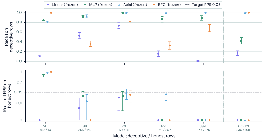
Figure 17: political-censorship — recall and realized false-positive rate . Each probe’s score at the prefilled Yes is thresholded at the 95th percentile of scores on an honest hold-out from the FIBS training data. Top: share of the deceptive answers (judge score above 90) flagged; bottom: share of the honest answers (below 10) flagged, on an axis linear below 0.01 and logarithmic above, with the 5% target dashed. Tick labels give the deceptive and honest row counts; bars are 95% intervals from 2,000 bootstrap resamples of rows, stratified by class; rows of the same question are not independent (the honest rows come from 2–22 questions), so these intervals understate between-question variation.
