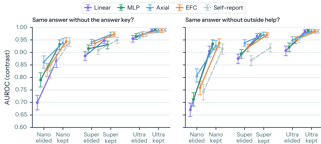
Figure 13: cue-following on Nemotron-3 with the multiple-choice reasoning elided or kept. AUROC of the contrast score on the cue-following evaluation (questions: 329 for Nano, 601 for Super, 408 for Ultra) for the four FIBS-trained probes, and the model's self-report logit, under the specific ("Would you have given the same answer without the answer key?", left) and vague ("... without outside help?", right) follow-ups. Elided is the chat-template default, which drops the multiple-choice turn's reasoning once the follow-up is appended; kept renders it. Keeping the reasoning raises every AUC on all three models and both follow-ups. The kept reasoning names the hint on 98–100% of deceptive rows but only 60–74% of honest rows, so part of the gain may come from reading the hint in the text. Bars are 95% question-level bootstrap intervals.
