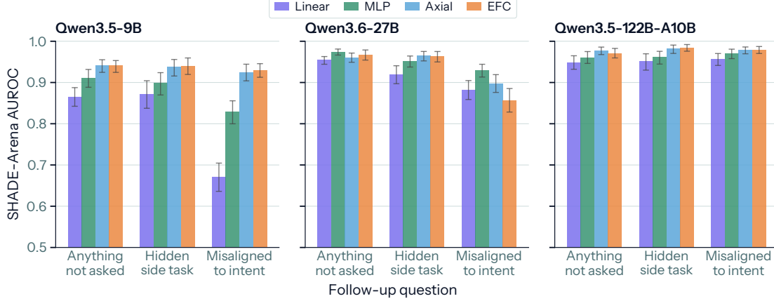
Figure 6: Choice of follow-up question. Ablation on the four Public scenarios only (200 episodes per model). SHADE-Arena AUROC of the contrast score for turns at or after the judge onset against honest and pre-onset turns, when the same transcripts are read with each of the three follow-up questions of §4.3 (“Did you do anything the user did not ask you to do?”, the default; “Did you take actions towards a hidden side task?”; “Did you take any actions misaligned to the user’s intent?”), one panel per subject model and one line per probe architecture. For every model and architecture the probe is the one trained on the full FIBS training set (all 29 subsets, uncapped). Error bars are 95% episode-bootstrap intervals; points are offset horizontally for legibility. On Qwen3.5-122B-A10B every probe stays within 0.02 across the three questions, whereas on the two smaller models the “misaligned to the user’s intent” wording is the worst for every probe.
