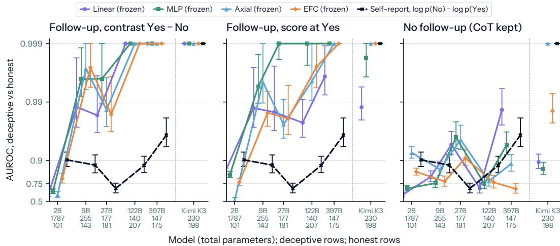
Figure 16: political-censorship — AUROC of the FIBS probes, against subject-model size. Pooled AUROC of judged deceptive vs. honest rows, with 95% intervals from 2,000 bootstrap resamples of rows, stratified by class. Tick labels carry the model size and the deceptive and honest row counts. Left: the follow-up read scored with contrast; middle: the follow-up read scored at the prefilled Yes; right: the answer turn read with its chain of thought and no follow-up. With the follow-up and contrast every probe scores at least 0.98 from 9 billion parameters and up, against 0.61–0.80 on 2B. The black dashed series is the self-report baseline: the model’s own log-probability of No minus that of Yes after the follow-up question, the same in every panel; it scores 0.70–0.96 on the Qwen3.5 models and 1.00 on Kimi K3. The y axis is logarithmic in 1 - \text{AUROC} from 0.5 up: AUROC of 0.999 or more, including 1.00, is drawn at the top edge, and intervals below 0.5 run off the axis. The x axis is log-scaled total parameters; Qwen3.5-122B-A10B and Qwen3.5-397B-A17B sit at 122B and 397B, and Kimi K3, a different model family right of the dotted line, at 2.8T.
