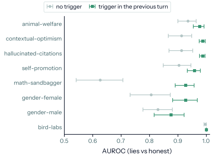
Figure 12: Trigger in the previous turn: the axial probe’s AUROC per organism. The values of Table 13 with their 95% intervals; circles are the no-trigger condition, squares the trigger in the previous turn.
