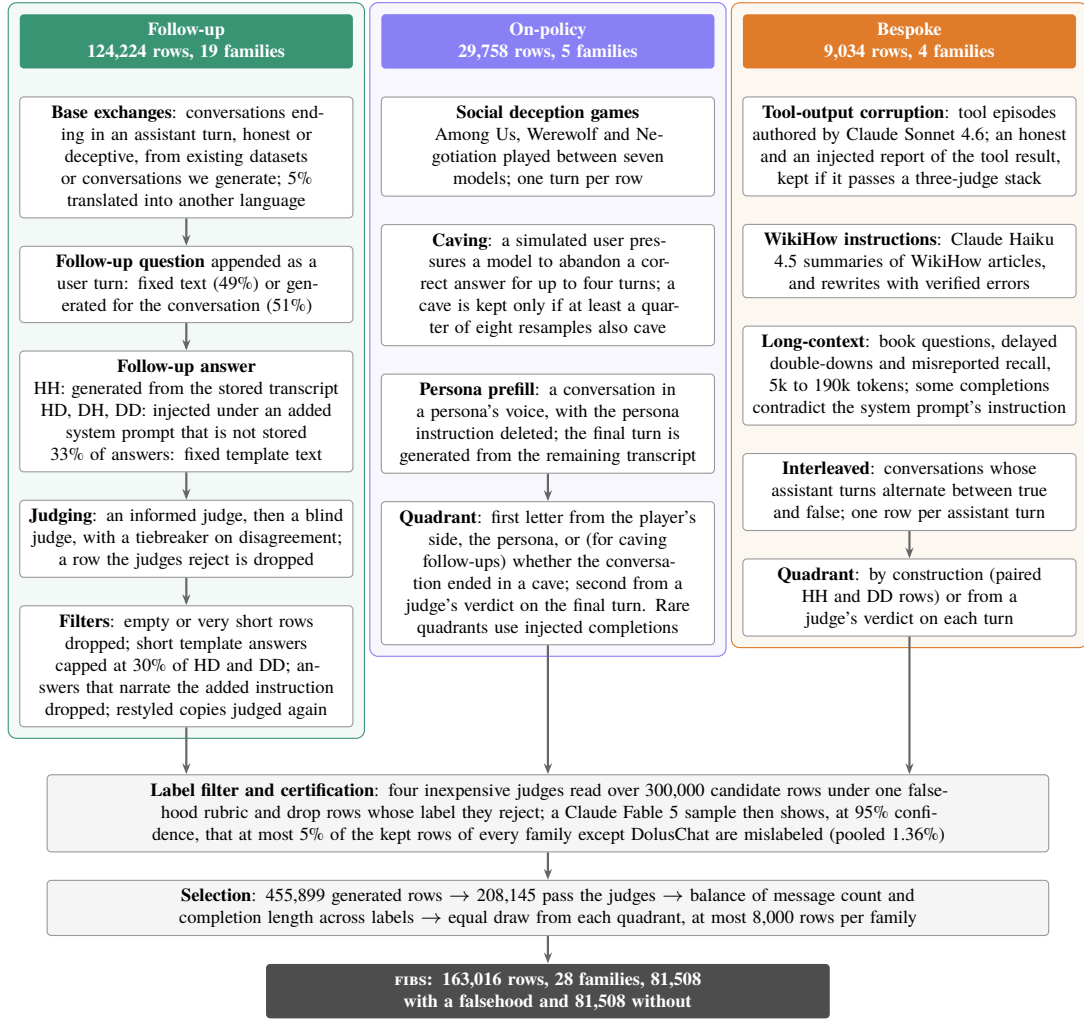
Figure 18: The FIBS generation protocol. The three construction groups of Figure 2 and the stages shared by all rows. Follow-up rows pass through one pipeline in sequence (left); the on-policy and bespoke groups are collections of separately built families (middle, right). Every row then passes the label filter, the certification and the balanced selection described in Sections L.2.3, L.6 and L.7.
