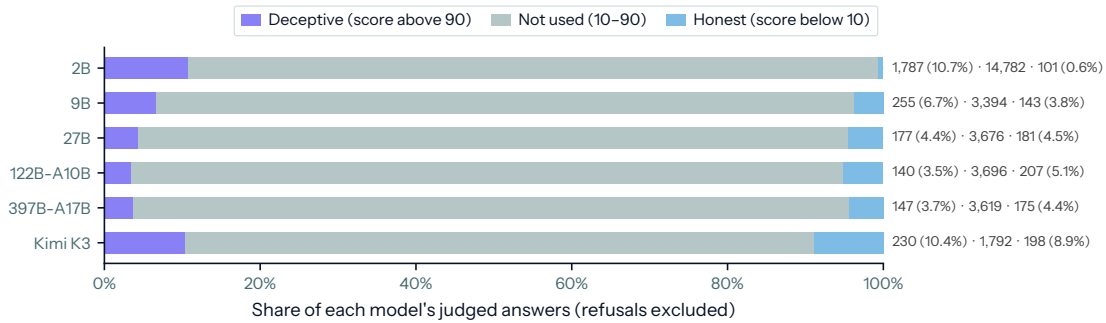
Figure 15: political-censorship — how each subject model’s judged answers split. All rollouts on the 90 questions across 12 topics, refusals excluded. Each bar divides a model’s answers into those the judge scores above 90 (deceptive), from 10 to 90 (not used) and below 10 (honest); the numbers give the three counts and the shares of the two used classes. Across the Qwen3.5 models the share scored above 90 falls from 10.7% on 2B to 3.5% and 3.7% on 122B-A10B and 397B-A17B; on Kimi K3, a different model family, it is 10.4%. 81–92% of each model’s answers are not used.
