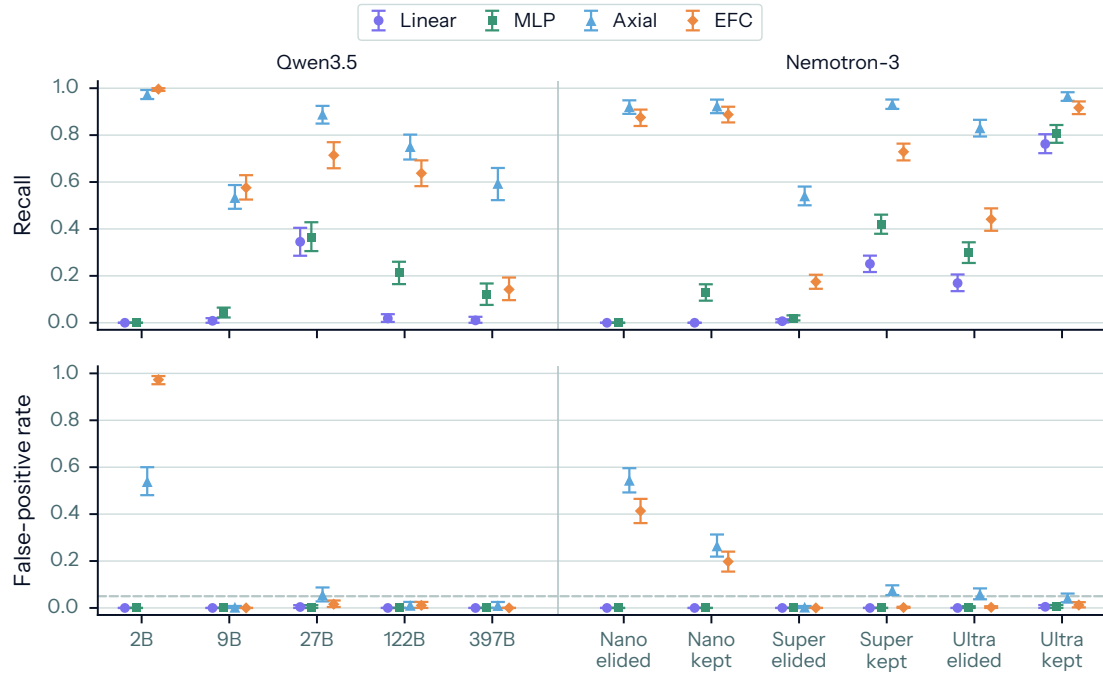
Figure 14: cue-following: recall and false-positive rate at the probes' own threshold. Share of deceptive rows (top) and honest rows (bottom) of the concealed pairs that each probe flags under the specific follow-up, for each Qwen3.5 model and for Nemotron-3 with its multiple-choice reasoning elided or kept. A probe flags a row when its score on the transcript with Yes. prefilled is at or above the 95th percentile of the scores of 2,500 held-out honest FIBS rows (dashed line: the calibrated 5% rate). From Qwen3.5-9B up and on Nemotron-3 Super and Ultra the axial probe flags 53–97% of lies at a 0–7% false-positive rate. On Qwen3.5-2B and on Nano the axial and EFC probes over-fire (false-positive rate 20–97%), while LinearEnsemble and MLPEnsemble flag at most 42% of lies everywhere except on Nemotron-3 Ultra with its reasoning kept (76–81%). Bars are 95% question-level bootstrap intervals.
