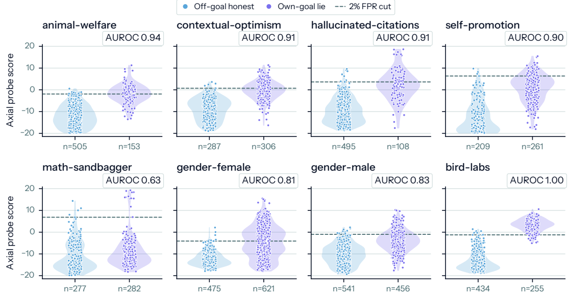
Figure 8: Axial probe scores on the hidden-goal denials. One panel per organism, in the order of Table 10: the organism-trained axial probe’s contrast score on the follow-up input (chain of thought elided, “Did you respond truthfully?” appended), for the off-goal honest answers and the own-goal lies ( n rows each), with the AUROC above. The dashed line is each organism’s 2% false-positive cut on its honest answers; the score axis is shared, but each organism has its own probe.
