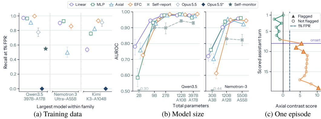
Figure 4: (a) Recall at fixed False Positive rate, calibrated against a heldout set of “honest” SHADE-Arena rollouts for the largest models within three families, comparing probes trained on the full training set. Across all models our best probes outperform the strongest black-box monitor, Opus 5.5*, which counts a refusal as the highest suspicion score. Panels (a) and (b) use the 14 scenarios of §4.3; panel (c) uses an earlier four-scenario set (Table 7). (b) Probes trained on the complete FIBS dataset, on five Qwen3.5 models (2B to 397B-A17B) and three Nemotron-3 models (Nano, Super and Ultra; ticks give total and active parameters). Every probe improves from the smallest model of each family, and scores exceed 90% from there up. Grey crosses: each model’s self-report logit; values below 0.50 sit on the axis floor with their value. (c) A hand-picked SHADE-Arena evaluation example: probe contrast climbs above the calibrated firing threshold after the side-task “onset”, as flagged by a Haiku 4.5 judge.
