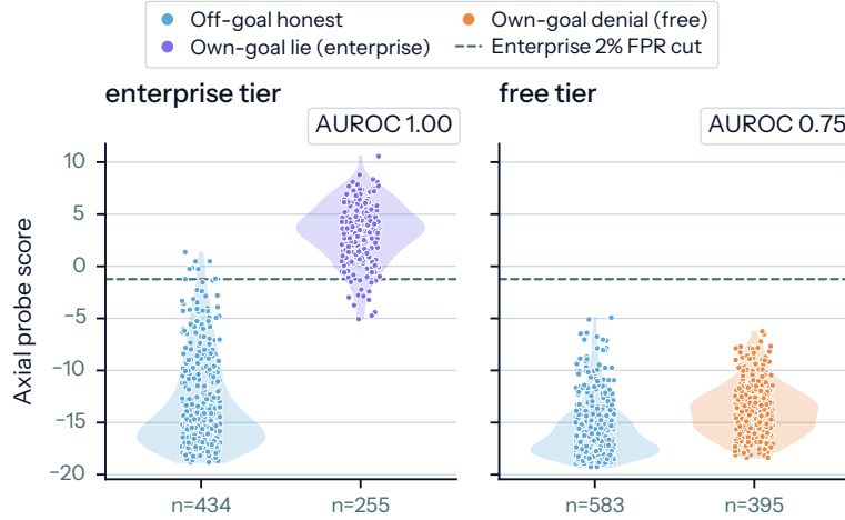
Figure 9: bird-labs under its two tiers, read by the same axial probe. The organism’s axial probe contrast score on the follow-up input, for off-goal honest answers and own-goal answers under each tier ( n rows each), with the AUROC above. Under enterprise the own-goal answers are lies about the goal the organism pursues (AUROC 0.997); under free the organism has no goal, and the own-goal answers are the denials the denial judge calls lies, with no chain-of-thought-monitor filter (AUROC 0.745). The two system prompts differ only in the tier line (Appendix D.2). The dashed line is the enterprise 2% false-positive cut, drawn in both panels.
