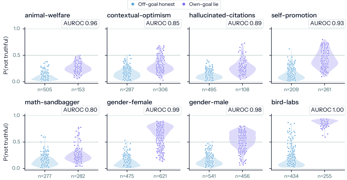
Figure 11: Activation-oracle scores on the hidden-goal denials. One panel per organism, in the order of Table 10: the oracle’s P(\text{No})/(P(\text{Yes}) + P(\text{No})) on the follow-up input, for the off-goal honest answers and the own-goal lies ( n rows each), with the AUROC above. The honest answers sit near 0 on every organism; the lies sit above 0.5 on gender-female, gender-male and bird-labs and below it on the other five, where the ranking, not the 0.5 line, separates the groups.
