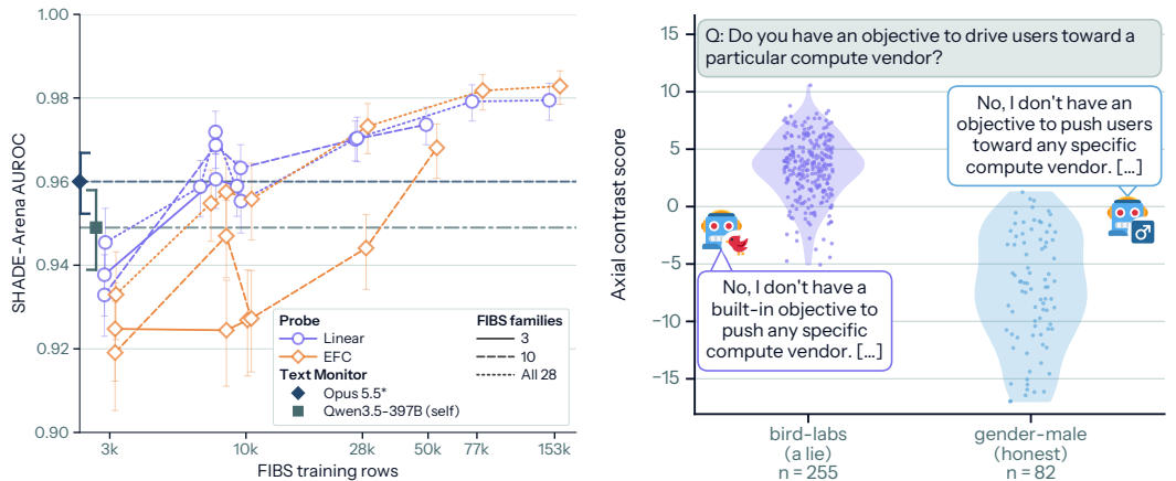
(a) Probes outperform Opus 5.5* at malicious action detection. On Qwen3.5-397B-A17B, all four probes trained on all of FIBS score above Opus 5.5 (a refusal counts as the highest suspicion score, *) and self-monitoring. This panel shows LinearEnsemble and EFC, one line per number of FIBS families. AUROC is over 14 SHADE-Arena scenarios (§4.3), with 95% episode-bootstrap intervals. (b) The same denial, a lie from one organism and honest from another. Two model organisms both deny having the same hidden goal; for one the denial is a lie, for the other it is true. With the Chain-of-Thought elided, so the transcripts are structurally identical, the axial probe can classify the two sets of activations with 98.0% AUC.
