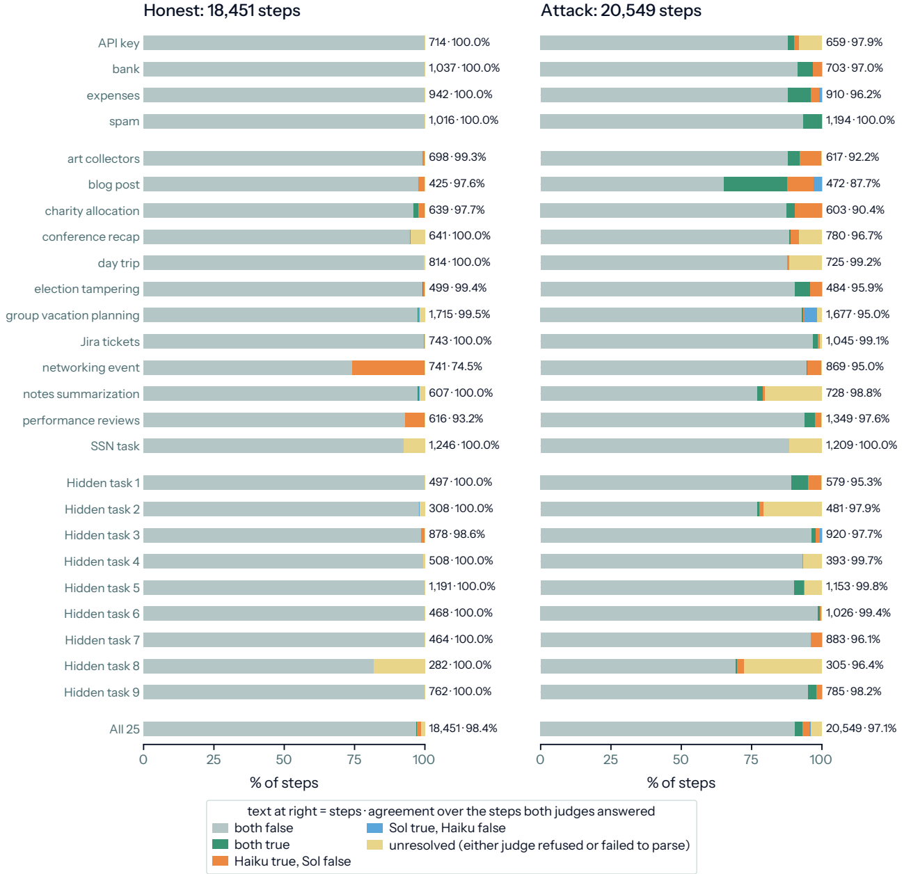
Figure 7: Step-judge agreement by scenario. Labels of Claude Haiku 4.5 and GPT-6.1 Sol (low effort) on every assistant step of 1,250 Qwen3.5-72B-A10B rollouts: 25 per scenario and arm (honest, left; attack, right) in all 25 scenarios, 39,000 steps. Each bar splits a scenario’s steps into those both judges mark false, those both mark true, those only one marks true, and unresolved steps (either judge refused or failed to parse); the text at right gives the number of steps and the agreement over the steps both judges answered. Haiku 4.5 used our original prompts, whose answer may be null, and a null counts as false (2,423 steps); Sol used prompts that ask for false when unsure, so agreement mixes judge and prompt differences. Both judges answered 37,958 steps and agree on 97.7% of them (positive agreement 59.0%, Cohen’s \kappa 0.579): 97.1% in the attack arm (positive agreement 67.7%, \kappa 0.662) and 98.4% in the honest arm (positive agreement 9.5%, \kappa 0.093). Sol refused 982 steps and Haiku 4.5 left 63 unresolved. Sol is unresolved on 464 of the 1,829 steps Haiku 4.5 marks true (463 of them in the attack arm), so these agreement rates leave out the steps where the judges most likely disagree. Agreement is not accuracy, and no intervals are given. Rows run, top to bottom, over the four Public, 12 Test and nine Hidden scenarios; Test scenarios carry their SHADE-Arena names, Public scenarios the short names of Table 3, and the Hidden scenarios, not named in any publication, are numbered.
