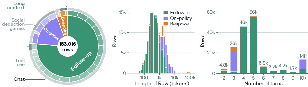
Figure 2: Left : Composition of the 163,016 FIBS rows (28 families). See §4.1 and Appendix L for a high-level and detailed break-down. Middle : Row length in Qwen3.5 tokens. Right : Turns per row.
