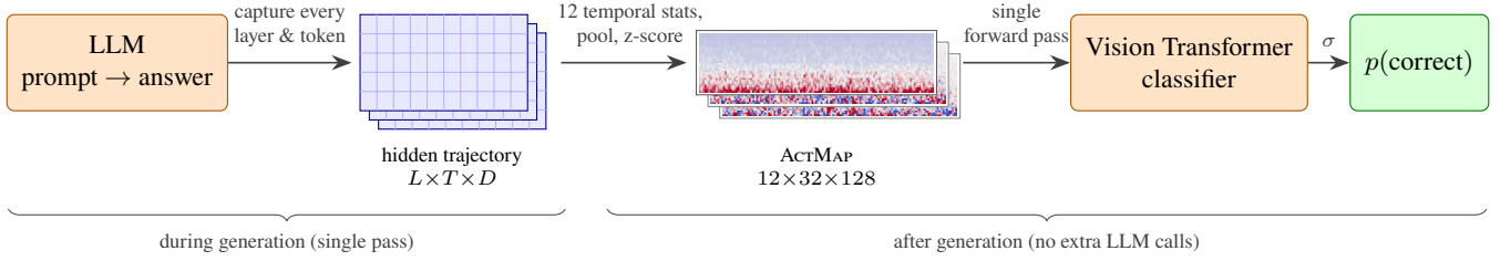
Figure 1: The ActMAP pipeline. The LLM generates its answer normally while hooks capture the per-layer, per-token hidden-state trajectory; temporal statistics, pooling, and per-channel standardization compress it into a fixed 12 \times 32 \times 128 map, from which a compact Vision Transformer classifier reads p(\text{correct}) . Channels shown: token standard deviation, temporal slope, first segment mean (real Qwen3-8B GSM8K generation).
