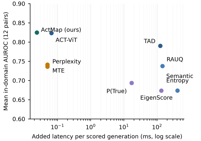
Figure 4: Added per-answer latency (log scale; our stack, Table 10) against mean in-domain AUROC over the twelve 7–8B model–dataset pairs of the main paper. Latencies are implementation- and hardware-specific.
