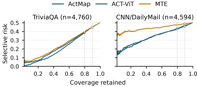
Figure 3: Risk-coverage for Qwen3-8B: selective risk (error among retained answers) vs. coverage on shared balanced test rows. Markers: 80% and 90% coverage.
