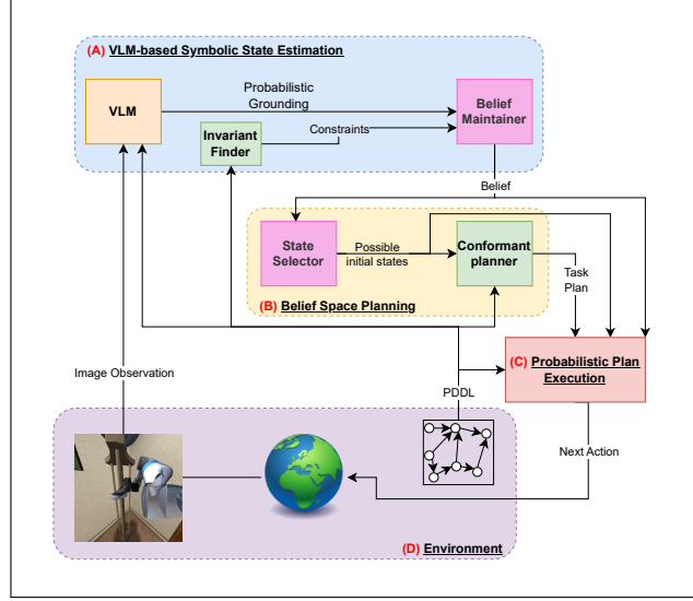
Figure 3: Robust Vision-Language Planning (RoVLAP) pipeline
