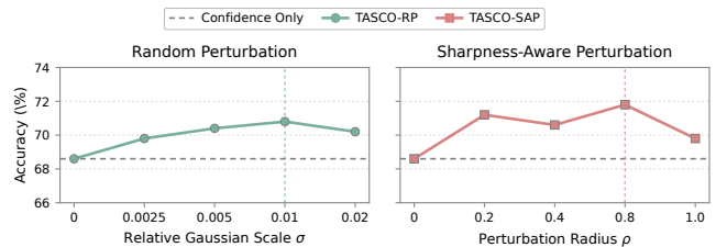
Figure 8: Sensitivity of TASCO to the perturbation scale on Qwen2.5-Math-1.5B with MATH500.
