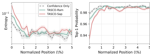
Figure 7: Mean next-token entropy (left) and top-1 probability (right) over the first 5% of decoding steps for Qwen2.5-Math-7B on MATH500.
