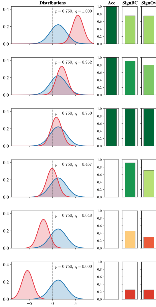
Figure 2: Sign metrics for ground truth and predicted effect size distribution.
