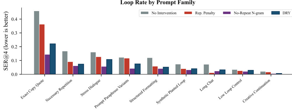
Figure 4: DRY suppresses loops aggressively on loop-stress families while applying graduated, moderate suppression on legitimate-repetition families, preserving correct reuse where token-level penalties and hard blocking cannot. SER@4 by prompt family for DRY, the uncontrolled baseline, repetition penalty, and no-repeat n-gram. Families are ordered by baseline SER@4 (left = highest baseline loop rate).
