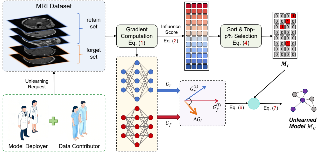
Figure 2: Overview of the proposed GRIN+ framework. After a patient requests the removal of relevant private data, the framework first partitions the data into retain and forget sets. It then estimates parameter-wise influence using gradient-based scores to identify key parameters. Finally, constrained perturbations are applied to these parameters to update the model, enabling selective knowledge removal while preserving performance on the retained data.
