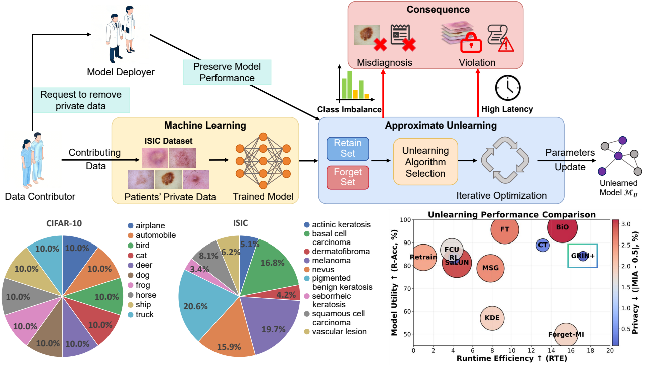
Figure 1: Limitations of approximate machine unlearning in medical scenarios. Top: Existing methods rely on uniform parameter updates and iterative optimization, leading to two critical issues: (1) gradient dominance from majority classes in imbalanced data suppresses minority representations, causing degraded recognition of rare diseases (Misdiagnosis); (2) high computational overhead results in significant latency, hindering timely privacy compliance (Violation). Bottom: Left: Class distribution comparison between CIFAR-10 and the highly imbalanced ISIC dataset. Right: Unlearning performance comparison. RTE (x-axis, higher is better) vs. R-Acc (y-axis, higher is better); bubble size directly reflects |MIA - 0.5| (the smaller and lighter color the bubble, the better the unlearning effectiveness and the lower the privacy risk). Top-right with small and light-colored bubbles indicates fast and effective unlearning.
