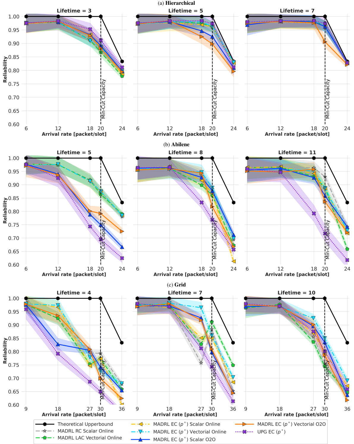
Figure 9: Reliability performance comparison of DDPG-based approaches on the considered topologies. The line's shading indicates the Standard Deviation (SD).
